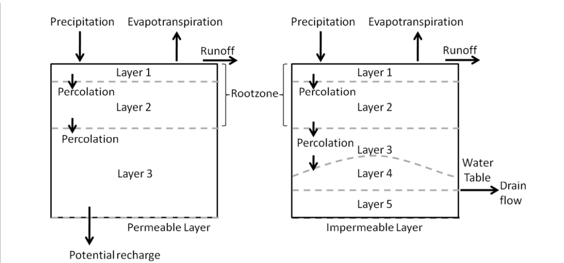
Figure 2 Schematic of the WaSim soil water balance model for (left) freely draining and (right) low permeability soils (modified from Hess and Counsell, 2000)
