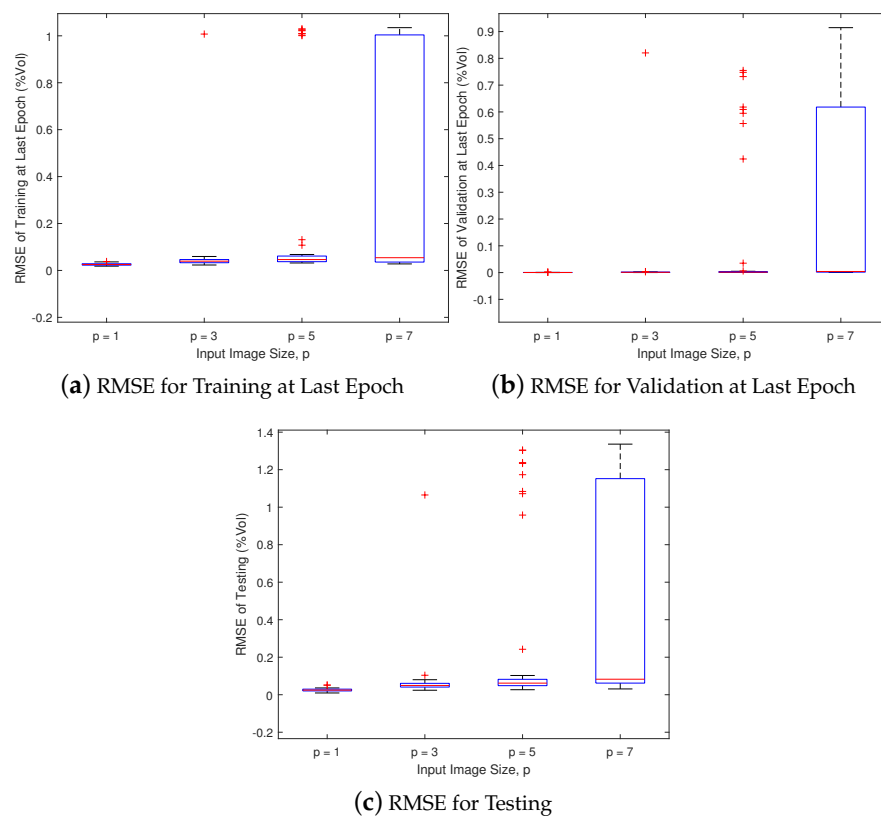
Figure 9. Training, validation, and testing results without errors on pixels for measurement points.
