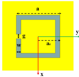
Figure 6: CSRR unit cell
