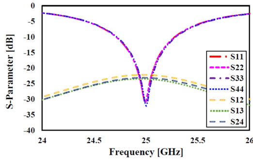
Figure 2: S- parameters of the proposed linear array
