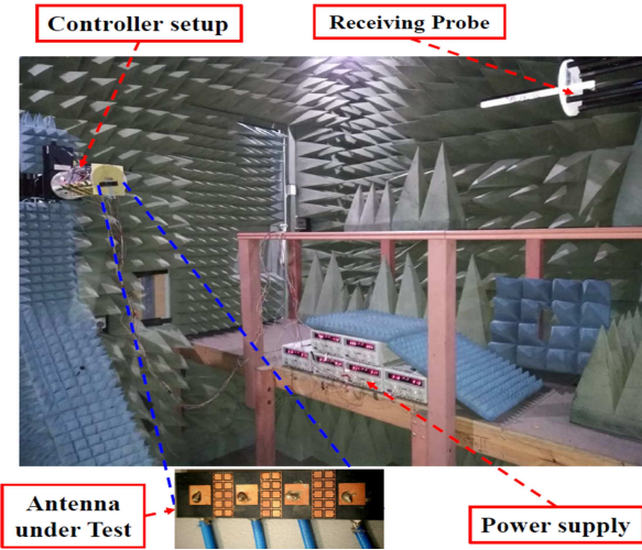
Figure 19: Measurement setup in anechoic chamber
