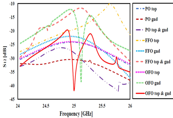
Figure 10: Mutual coupling ( S_{12} ) between antenna array with different CSRR configurations
