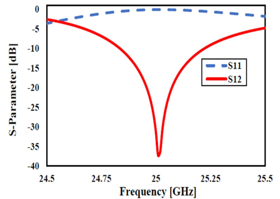
(a) Scattering parameter response
