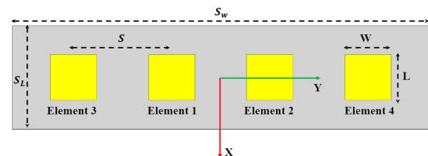
Figure 1: Four elements linear array
