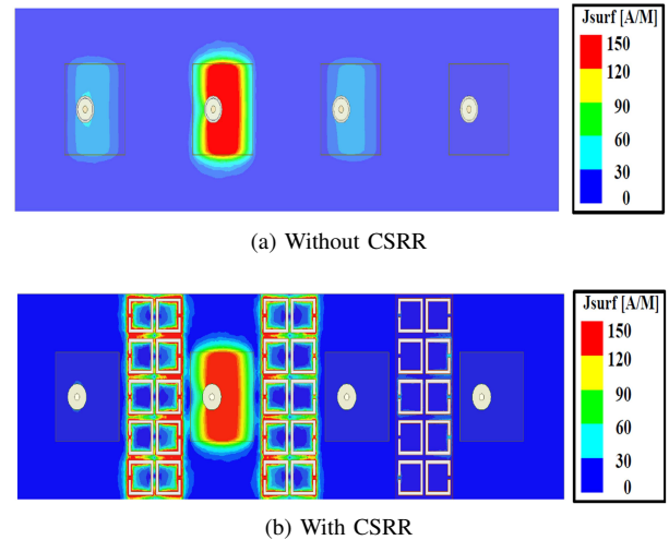
Figure 13: Current distribution in four-element antenna array
