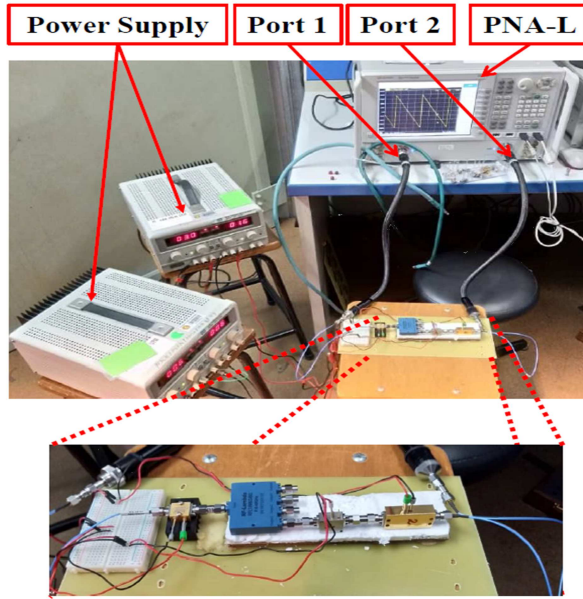
Figure 18: Feed network measurement setup
