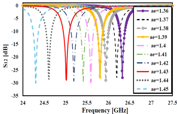
Figure 7: S_{12} for different values of ' a '
