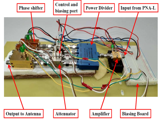
(b) Real time setup
