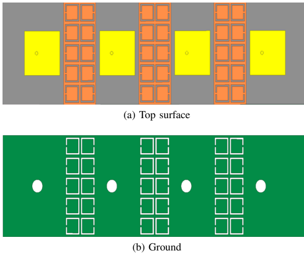
Figure 11: Antenna array with opposite faced CSRR elements
