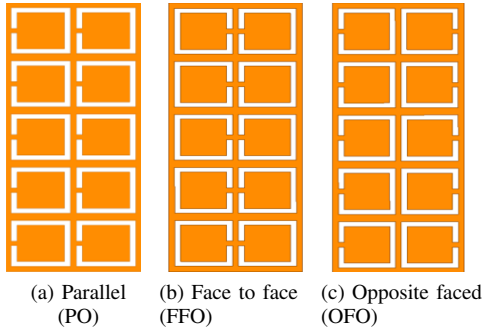
Figure 9: Different orientation of CSRR elements
