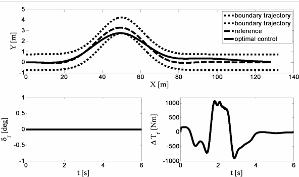
Fig. 7. TVD optimization results for roll minimization case ( \mu = 1 ).
