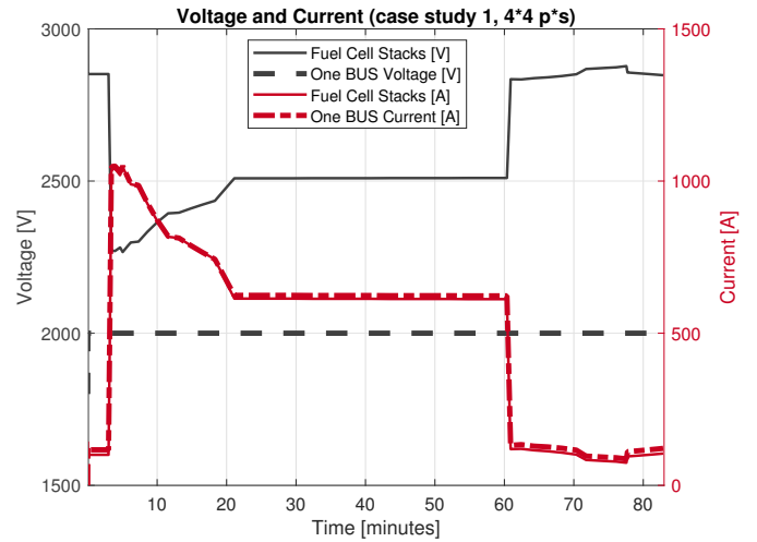
(c) Voltage and current values of healthy stacks.
