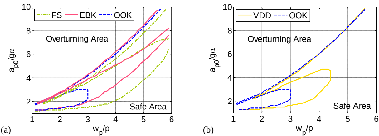
Fig.12. Overturning spectra of BLC05 evaluated for different restraint conditions: free-standing (FS); anchorages with elastic-brittle stiffness (EBK); anchorages with on-off stiffness (OOK); viscous damper devices (VDD).
