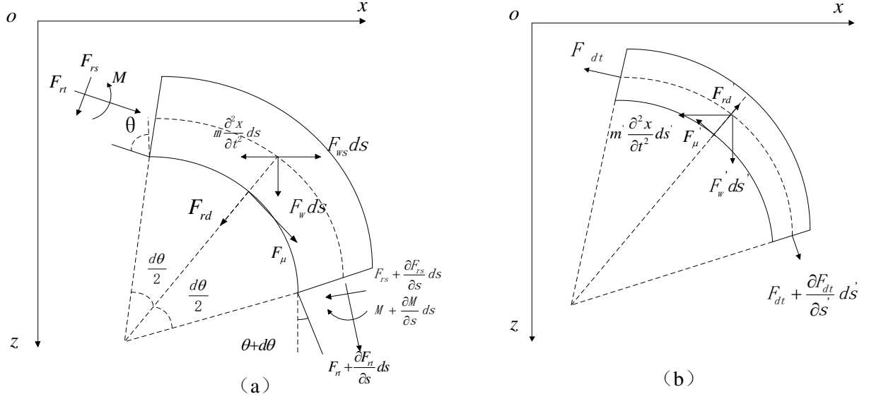
Fig.2 Mechanical models of the micro elements: (a) the riser; (b) the CT.
