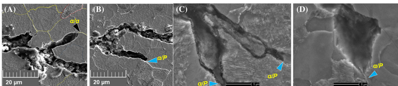
FIGURE 20 Phases influencing fatigue crack growth rate in J2N steel in seawater [Colour figure can be viewed at wileyonlinelibrary.com ]
