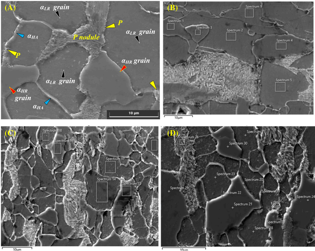
FIGURE 5 Energy-dispersive x-ray analysis of phase composition in S355J2 + N steel in the rolling direction [Colour figure can be viewed at wileyonlinelibrary.com ]
