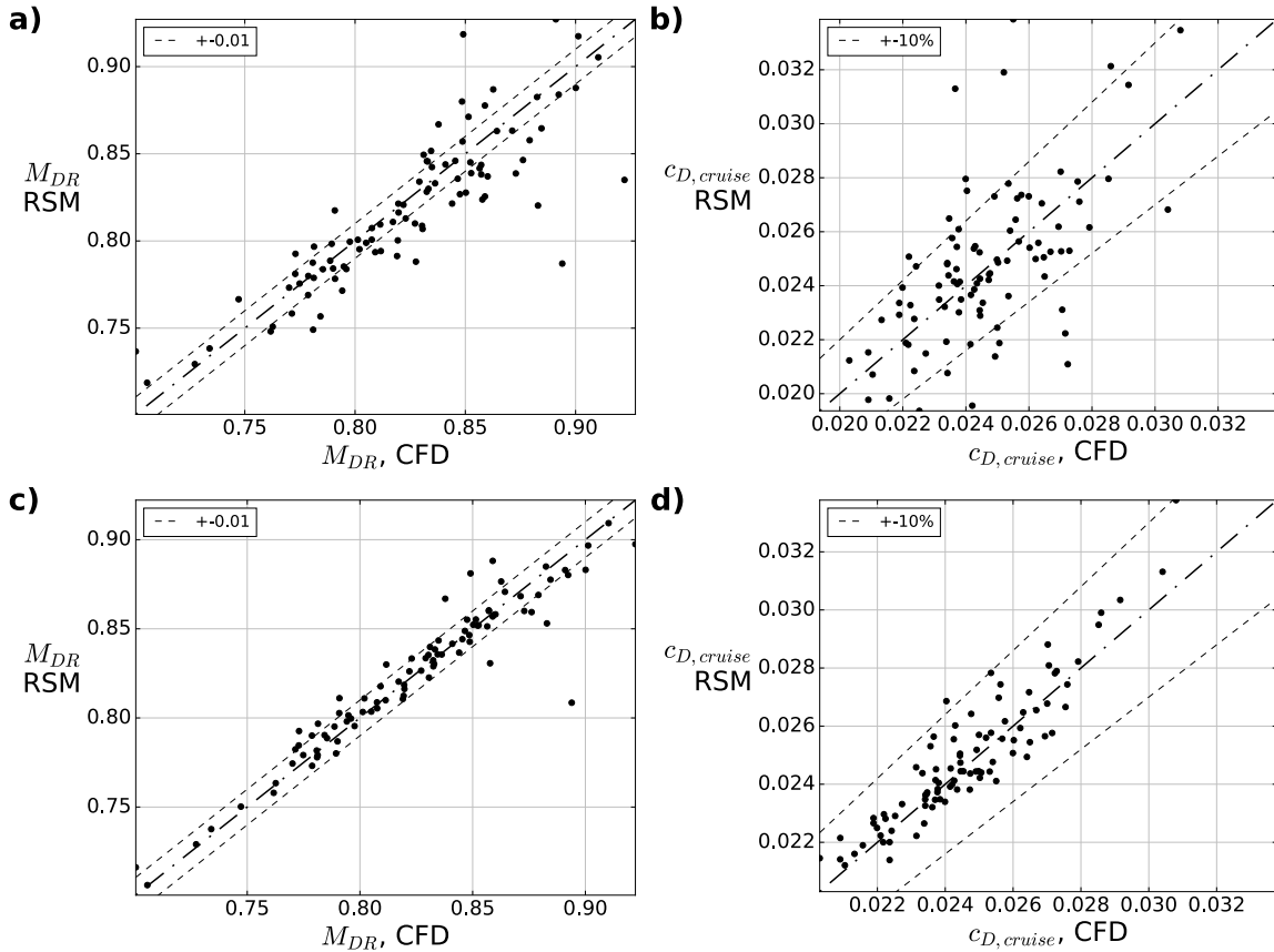
Fig. 10. Validation against an independent data set, predictions from RSM compared to CFD results. (a) Drag-rise Mach number at MF_{CR} = 0.75 from a simple Gaussian process model; (b) drag at cruise conditions (Eq. (2)) from a simple Gaussian process model; (c) and (d) use the combined RSM developed in this paper.
