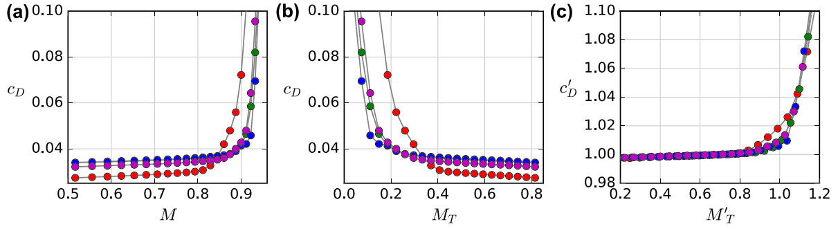
Fig. 6. Four example drag-rise curves, sampled at maximum MFCR . (a) Raw input data, c_D against M ; (b) c_D against M_T ; (c) transformed and normalized to c_{D,ref} and M_{ref,T} as function of M'_T .
