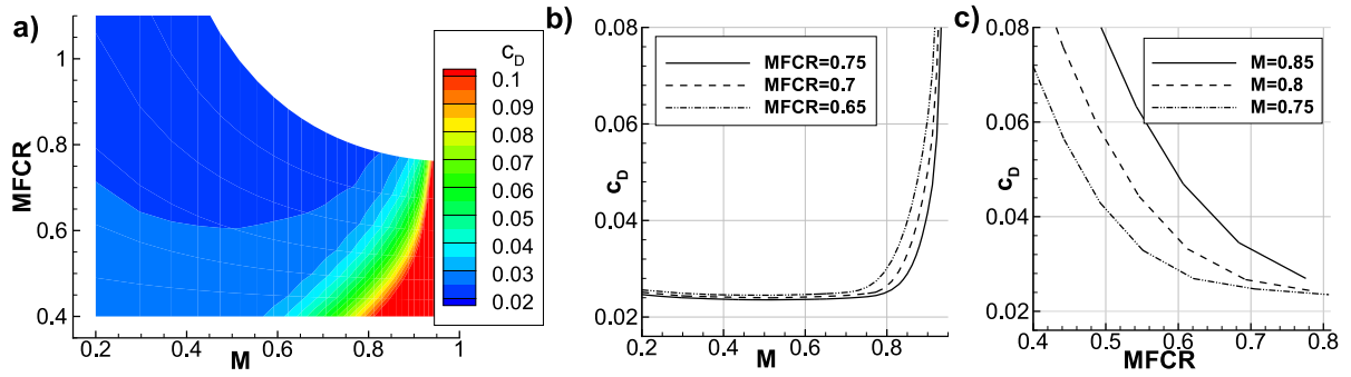
Fig. 1. (a) Drag map of an example nacelle. (b) c_D as a function of M (“drag-rise curves”) at constant MFCR . (c) c_D as a function of MFCR (“spillage curves”) at constant M . Drag coefficients use highlight area as reference area.
