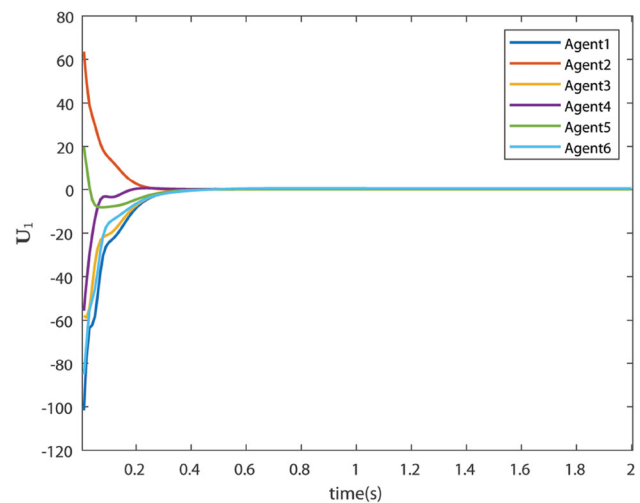
Fig. 3 Control U_1 (Case 1)
