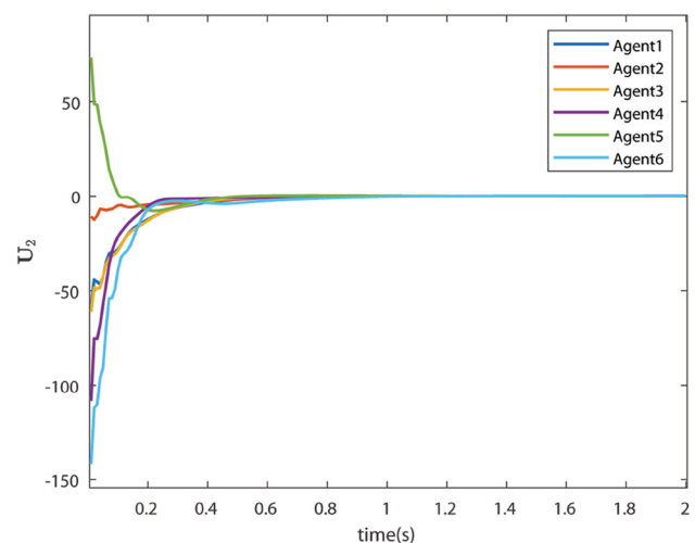
Fig. 4 Control U_2 (Case 1)
