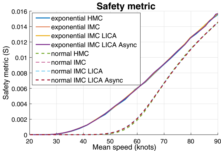
Figure 12. Safety metric as a function of mean speed for all algorithms. (Threshold time: 60s. Agent density: 165 agents.)
