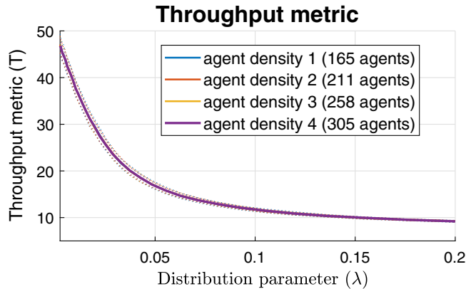
Figure 3. Throughput metric as a function of the exponential distribution parameter ( \lambda ) for the HMC algorithm. (Threshold time: 60s. Dotted lines show the standard deviation. The distribution parameter is related to the speed distribution of vehicles.)
