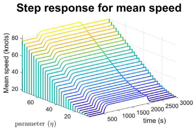
Figure 37. Step response for mean speed with normal distribution (Algorithm: IMC for steady-state, HMC for transitions. The distribution parameter is related to the speed distribution of vehicles).
