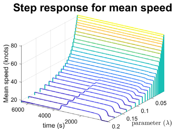
Figure 38. Step response for mean speed with exponential distribution (Algorithm: IMC for steady-state, HMC for transitions. The distribution parameter is related to the speed distribution of vehicles).
