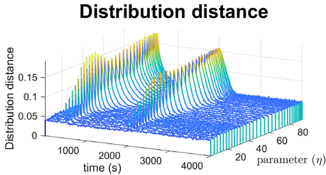
Figure 36. Distribution distance transitioning from a normal to an exponential distribution (at t = 500\text{s} ) and back (at t = 2,000\text{s} ). (Threshold time: 60s. Algorithm: HMC. Agent number: 165. The distribution parameter is related to the speed distribution of vehicles.)
