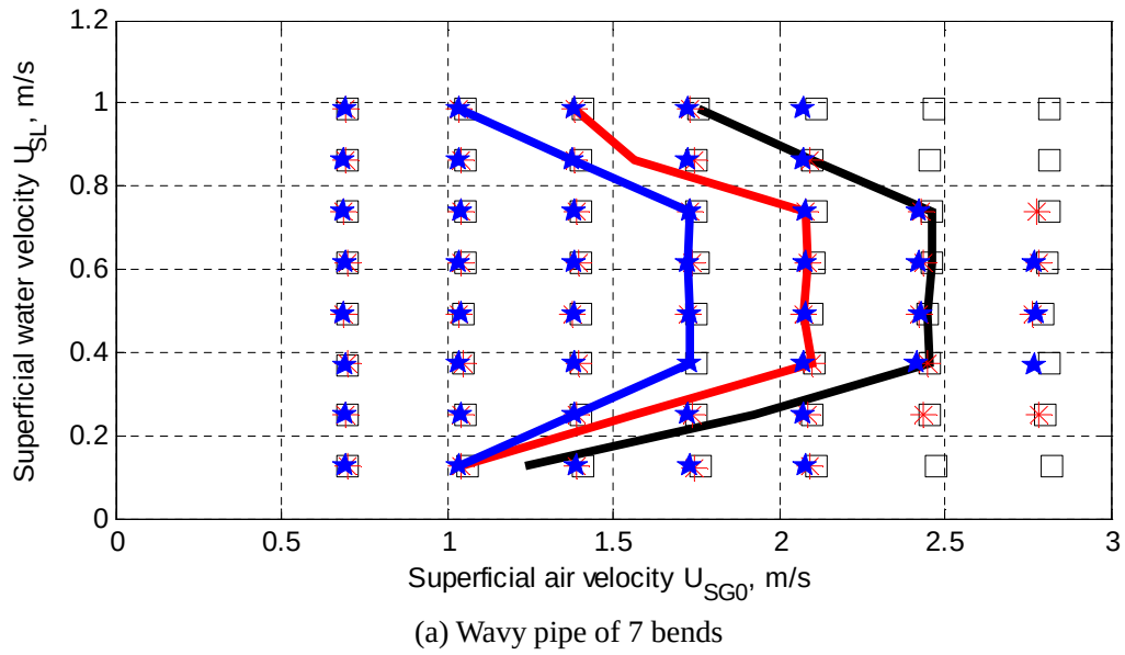
Fig. 6 Stability boundaries for the 2" and 4" plain riser and pipeline/wavy-pipe/riser systems
