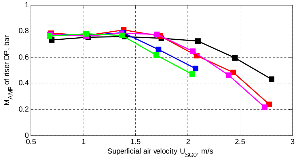
(a) U_{SL} = 0.25 m/s
