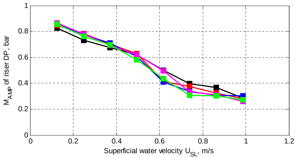
(c) U_{SG0} = 0.70 m/s
