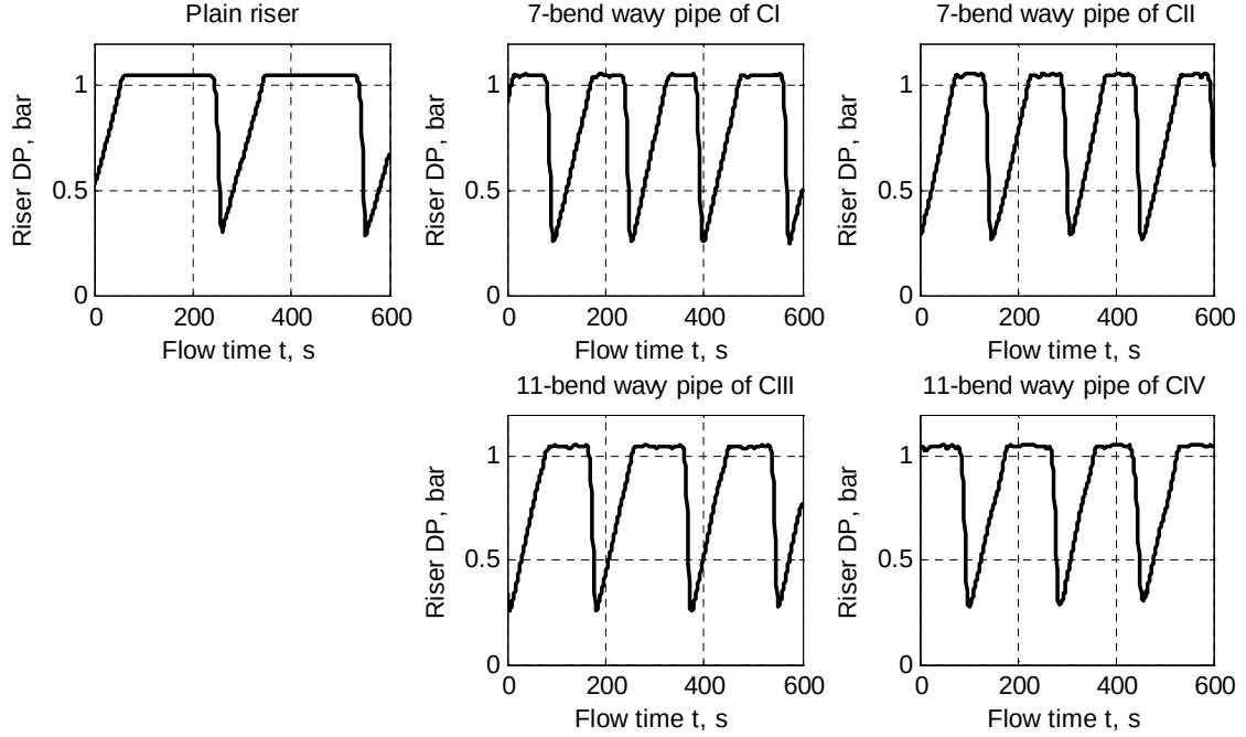
Fig. 10 Riser DP time traces of SS for the 2" plain riser and pipeline/wavy-pipe/riser systems of different test configurations ( U_{SG0} = 0.70 m/s, U_{SL} = 0.25 m/s)
