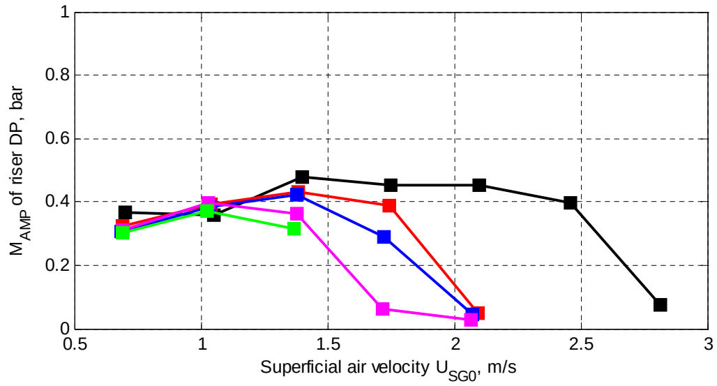
(b) U_{SL} = 0.86 m/s
