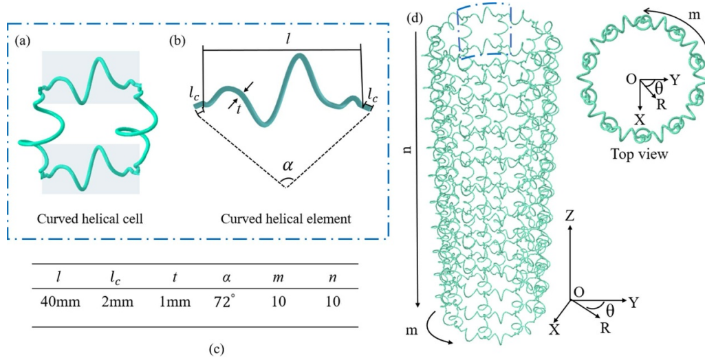
Figure 1. Dimension of cylindrical helical cell metamaterial, (a) curved helical cell, (b) curved optimised spring element, (c) parameters for curved optimised spring element and cylindrical metamaterial, (d) cylindrical helical cell metamaterial.
