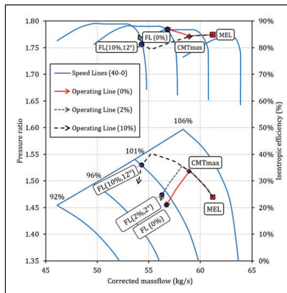
Figure 19. Operating points of last lumped stages during ramp-up. CMT: combustor mean temperature; FL: full load; MEL: minimum environmental load.
