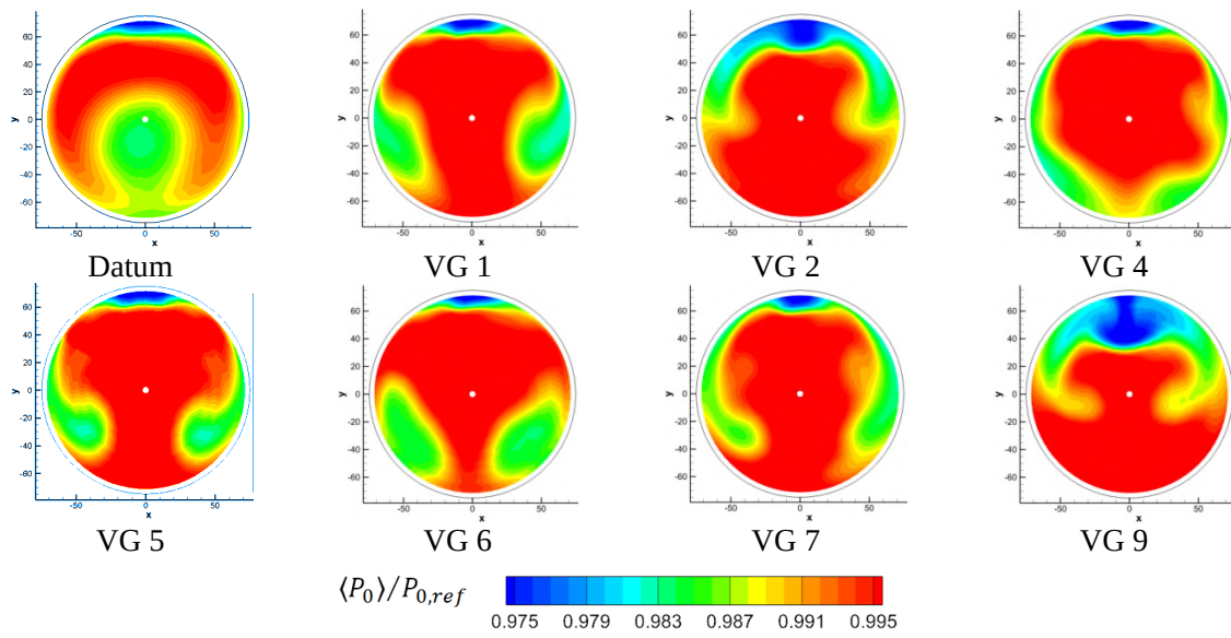
Figure 9. Time averaged total pressure distributions at Min = 0.27
