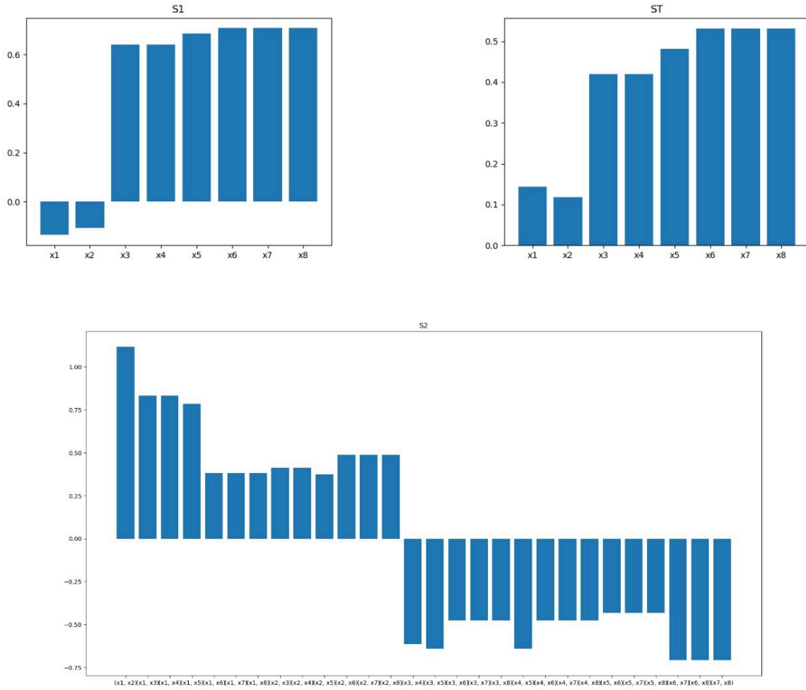
Fig. 13 CD Sobol's indices.
