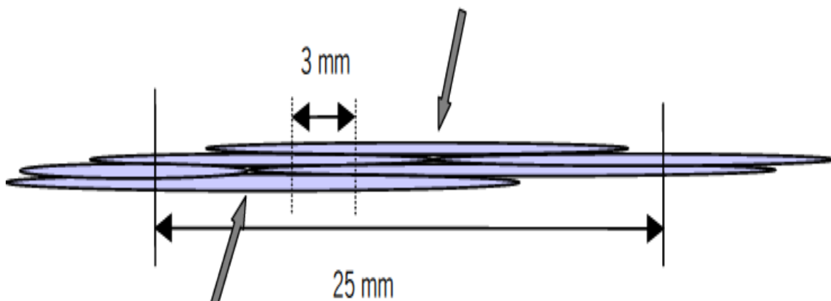
Figure 3. Schematic representation of failure mechanism of flax fibres. At 25 mm clamping length, elementary fibres slip over each other. At 3 mm, cracks run through the cross section of the elementary fibres. Adapted with permission from [16]. Copyright 2013 by Eindhoven University.
