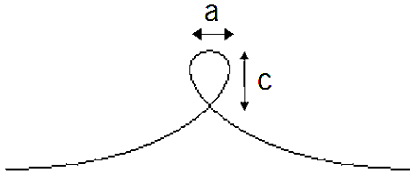
Figure 4. Loop test for compression. The ratio c/a changes at failure point.
