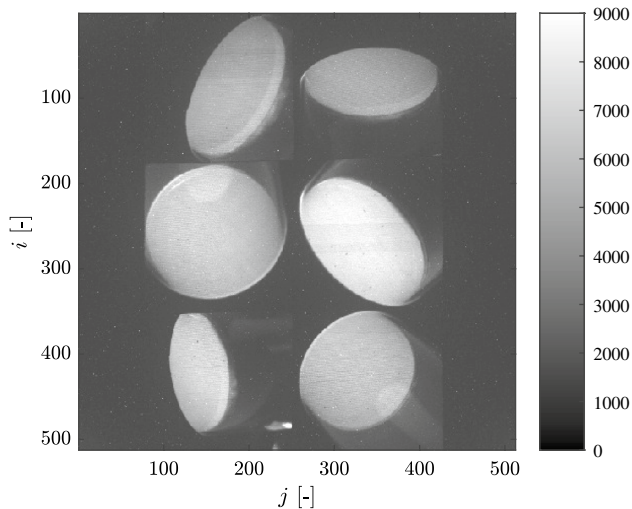
Fig. 4 Raw FRS image acquired at the optimised wavenumber of 18,788.455 \text{ cm}^{-1}
