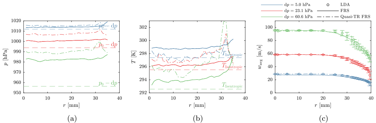
Fig. 8 Radially averaged pressure profiles with p_0 - dp (dashed) (a), temperature profiles with isentropic temperature (dashed) (b) and axial velocity profiles (solid) with LDA measurements (circle) (c) for frequency scanning (solid) and quasi-time-resolved data analysis
