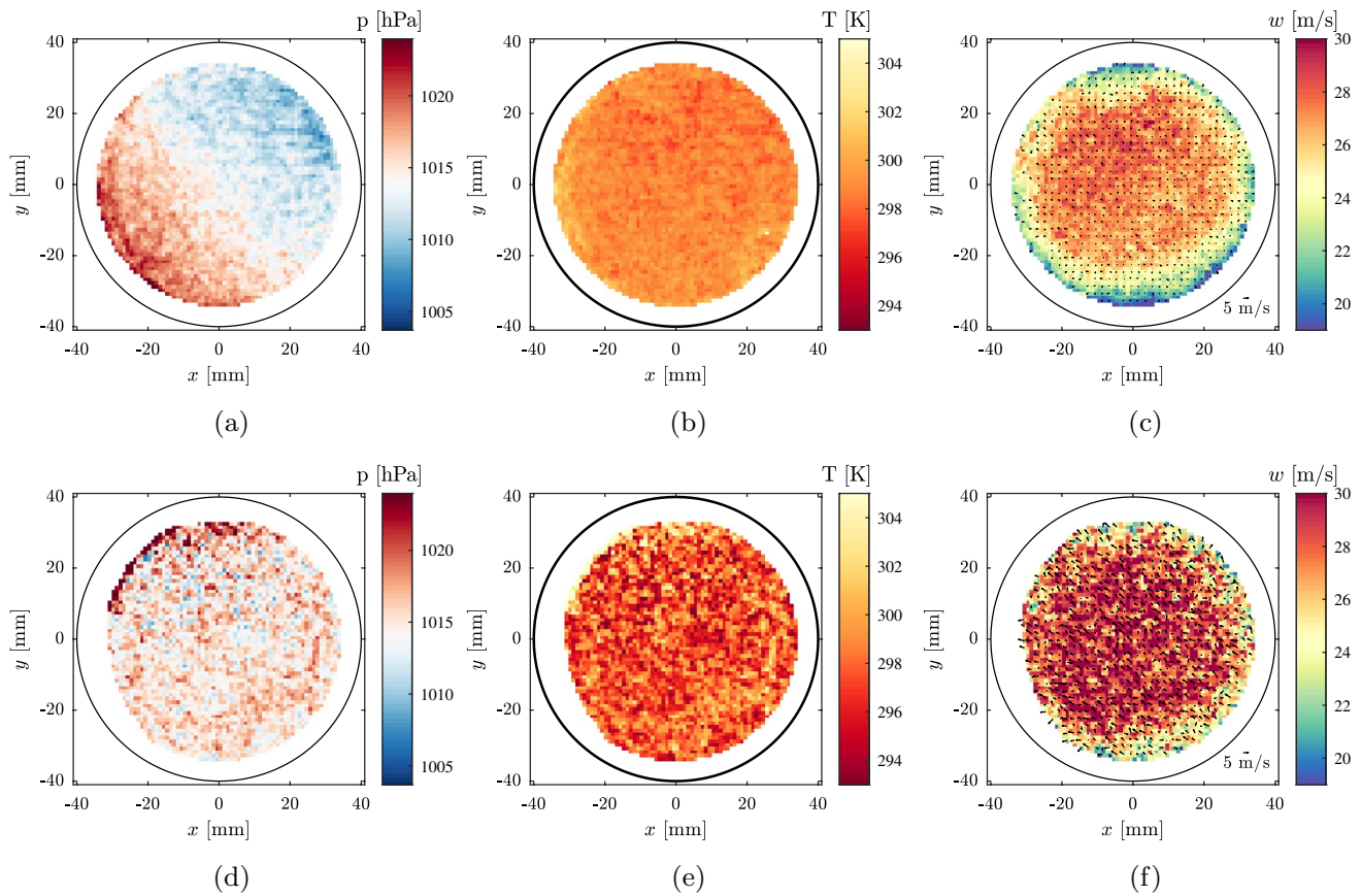
Fig. 7 Comparison of time-averaged and quasi-time-resolved maps of the straight pipe flow for pressure (a, d), temperature (b, e) and axial velocity maps (c, f) for dp = 5 hPa. The in-plane velocity com-
