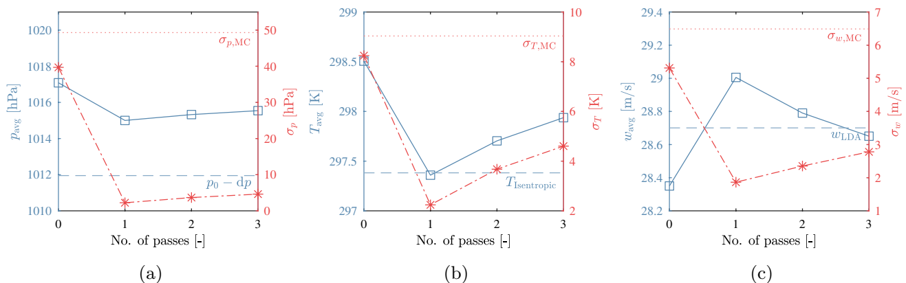
Fig. 9 Spatial averages (blue, solid) and standard deviations \sigma (red, dashed-dotted) of the constant core flow region at operating point dp = 5.0 hPa plotted against the number of multistage passes (zero means conventional fitting) for p (a), T (b) and w (c). Reference val-
