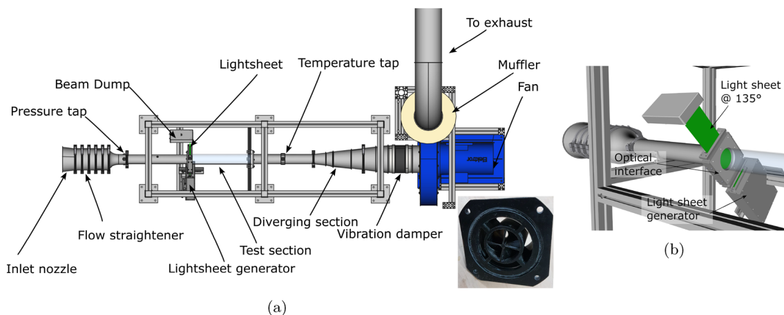
Fig. 2 a Schematic of the aspirated pipe flow facility. The inset on the right shows a photograph of the axial swirler. b Enlarged view of the test section with light sheet interface
