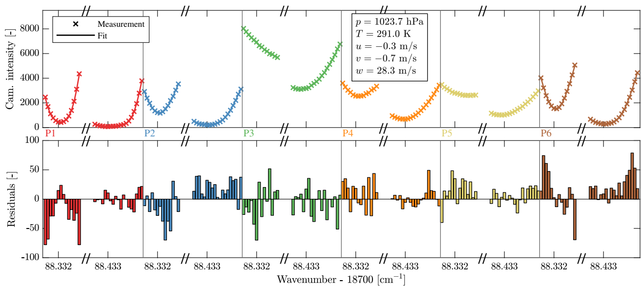
Fig. 6 Top Evaluation of FRS intensity spectra obtained from frequency scanning for a single super-resolution element. Each colour represents a different perspective. The measured FRS intensities
