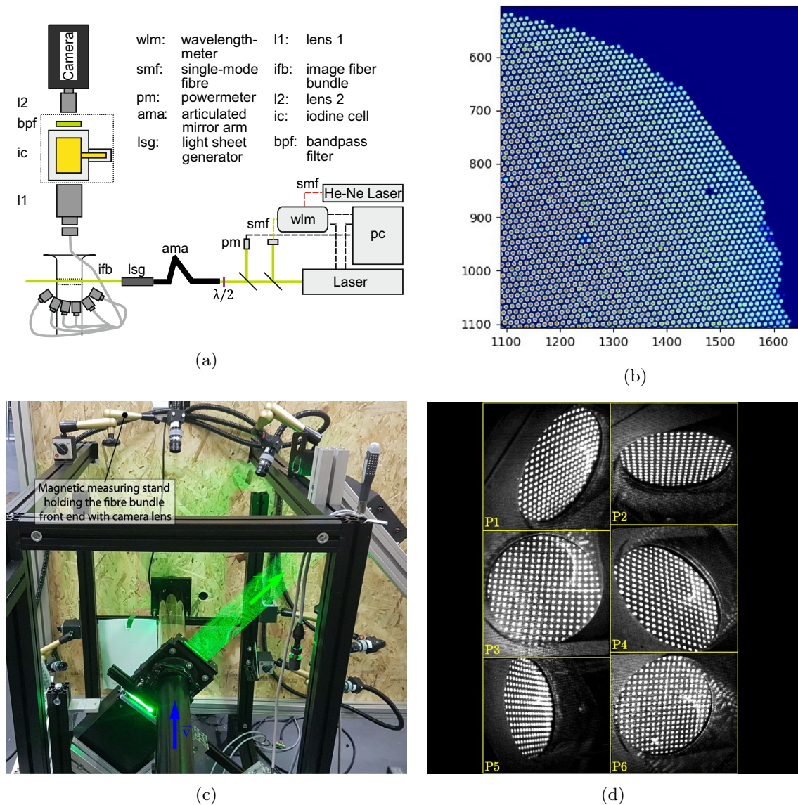
Fig. 3 a Principle layout of the FRS system. b Close-up image of a fibre bundle exit illuminated with an integrating sphere. c Photograph of the FRS instrumentation installed at the flow facility. d Snapshot of a calibration target observed through the six-branch image fibre bundle
