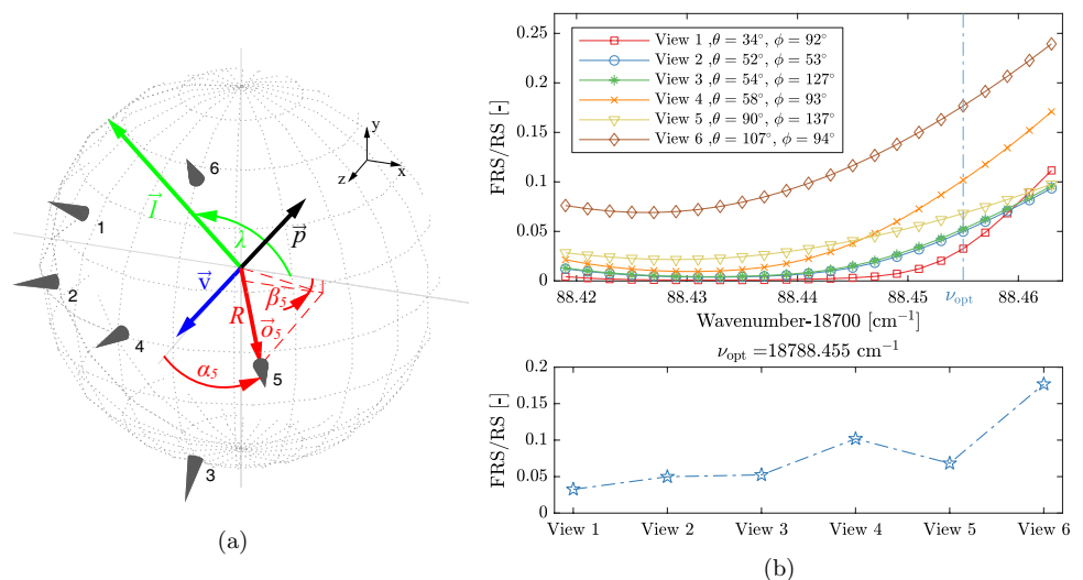
Fig. 1 a Orientation of the six optimised camera views on a sphere around the region of interest. b Top Simulated FRS intensity spectra normalised by the available Rayleigh scattering (RS) for a frequency scan around the 18788.44 \text{ cm}^{-1} -doublet for the six optimised camera views. The scattering angles \theta and \phi are indicated in the legend. Bottom FRS signal intensities at the optimised single-pulse wavenumber \nu_{\text{opt}}
