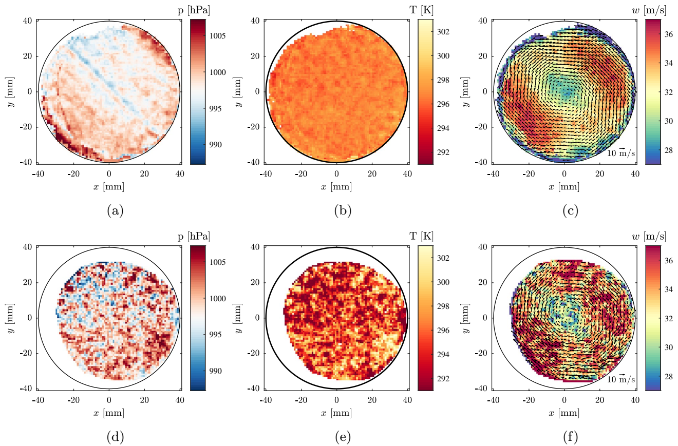
Fig. 10 Comparison of time-averaged and quasi-time-resolved maps of the swirling flow for pressure ( a , d ), temperature ( b , e ) and axial velocity maps ( c , f ) for dp = 26 hPa. The in-plane velocity compo-
