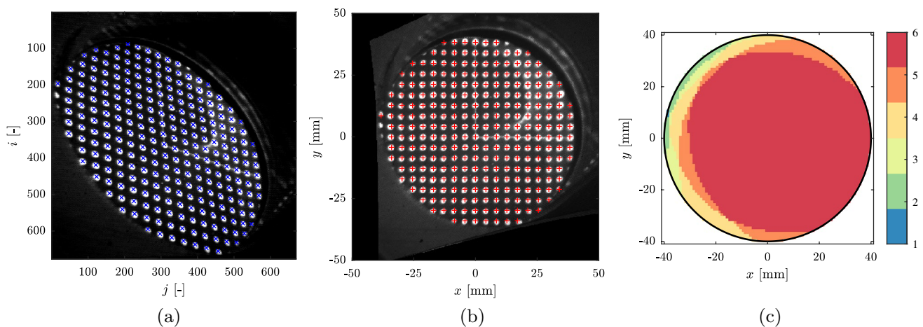
Fig. 5 Image transformation of perspective #4 from camera coordinate system (a, blue cross) to world coordinate system (b, red plus). c Parts of the duct (black, solid) are obstructed from view. The number of views having optical access to a particular area is indicated by the contours
