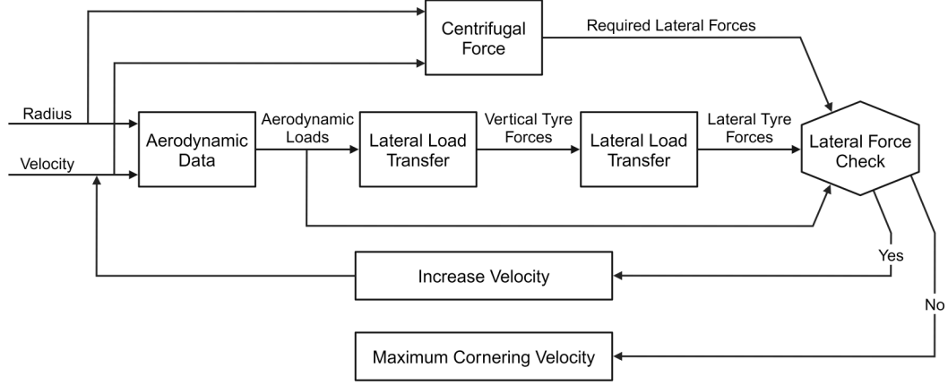
Figure 7: Vehicle dynamics model procedure
