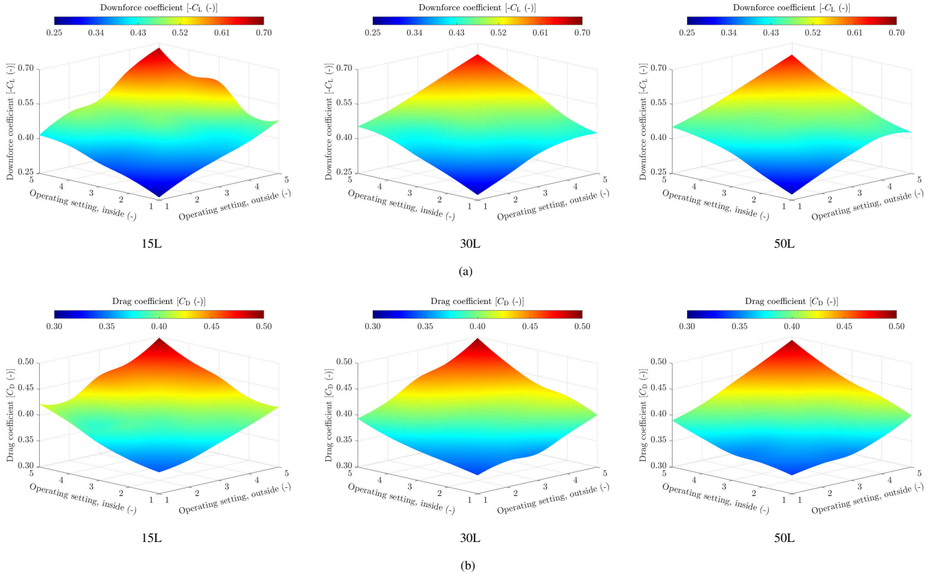
Figure 22: (a) Downforce coefficients and (b) drag coefficients as a function of the operating settings for the inside and outside located active aerodynamic devices of the tilted rear wing high-performance vehicle concept in various cornering conditions
