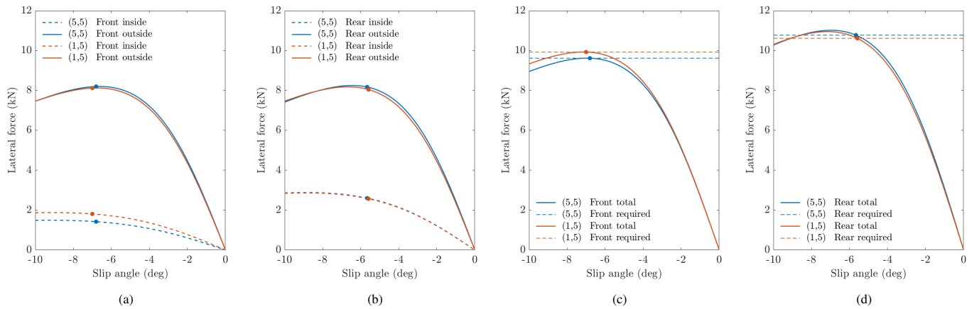
Figure 28: Comparison between the lateral forces produced by the (a) front tyres, (b) rear tyres, (c) front tyres combined, and (d) rear tyres combined of the tilted rear wing high-performance vehicle concept in its maximum symmetric (5,5) and optimal inside bias (1,5) operating states in the 50L radius corner
