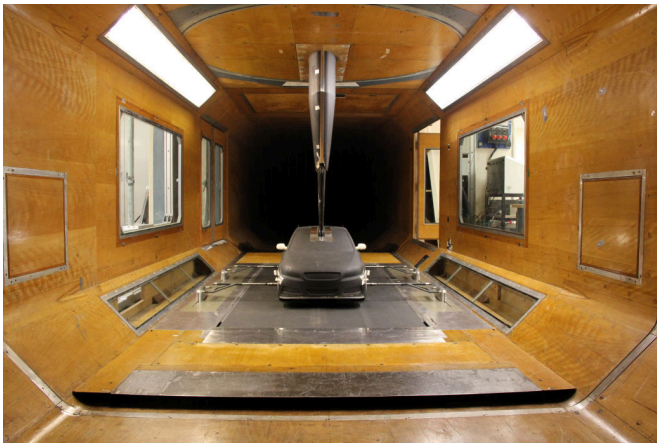
Figure 3: 35% scale DrivAer hp-F model in the 8x6 Wind Tunnel using the moving ground setup at Cranfield University. Reproduced from [Rijns, S., Teschner, T.-R., Blackburn, K., Brighton, J., "Effects of cornering conditions on the aerodynamic characteristics of a high-performance vehicle and its rear wing", Physics of Fluids , 36(4), 045119 (2024).], with the permission of AIP Publishing.
