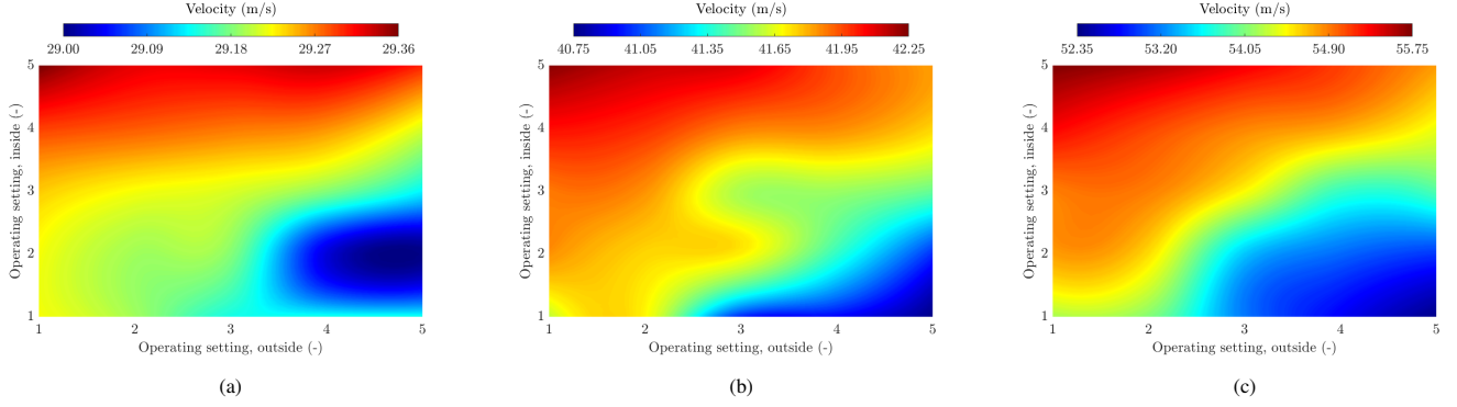
Figure 27: Maximum velocity as a function of the operating settings for the inside and outside located active aerodynamic devices of the tilted rear wing high-performance vehicle concept in the (a) 15L radius corner, (b) 30L radius corner, and (c) 50L radius corner
