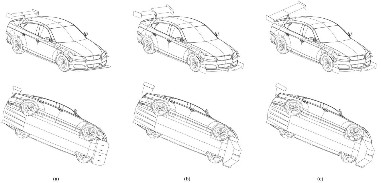
Figure 2: (a) baseline vehicle: DrivAer hp-F with standard rear wing, (b) split wing concept: DrivAer hp-F with active split front wing and split rear wing, and (c) tilted wing concept: DrivAer hp-F with active split front wing and tilted rear wing. The two active high-performance vehicle concepts are depicted in an asymmetric operating setting to illustrate the designs
