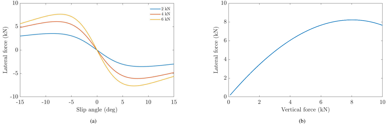
Figure 10: (a) Lateral tyre force as a function of slip angle, and (b) lateral tyre force as a function of vertical force at a constant slip angle of \alpha = -7^\circ
