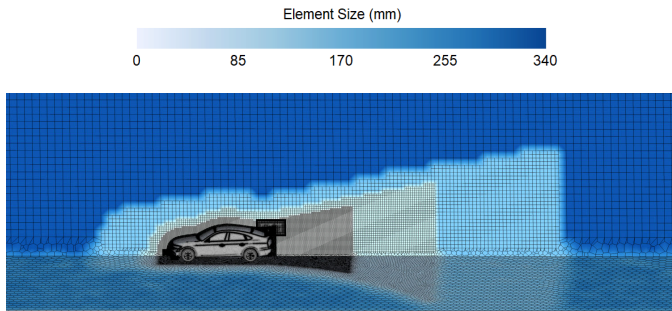
Figure 6: Element sizes in proximity of the vehicle using a slice at y = 0 mm (symmetry) for illustration
