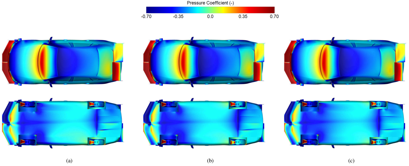
Figure 17: Pressure coefficient distribution on the split rear wing high-performance vehicle concept in its maximum inside bias operating state (1,5) in the (a) 15L radius corner, (b) 30L radius corner, and (c) 50L radius corner
