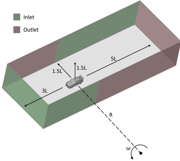
Figure 4: Computational domain with cornering boundary conditions. Reproduced from [Rijns, S., Teschner, T.-R., Blackburn, K., Brighton, J., "Effects of cornering conditions on the aerodynamic characteristics of a high-performance vehicle and its rear wing", Physics of Fluids , 36(4), 045119 (2024).], with the permission of AIP Publishing.
