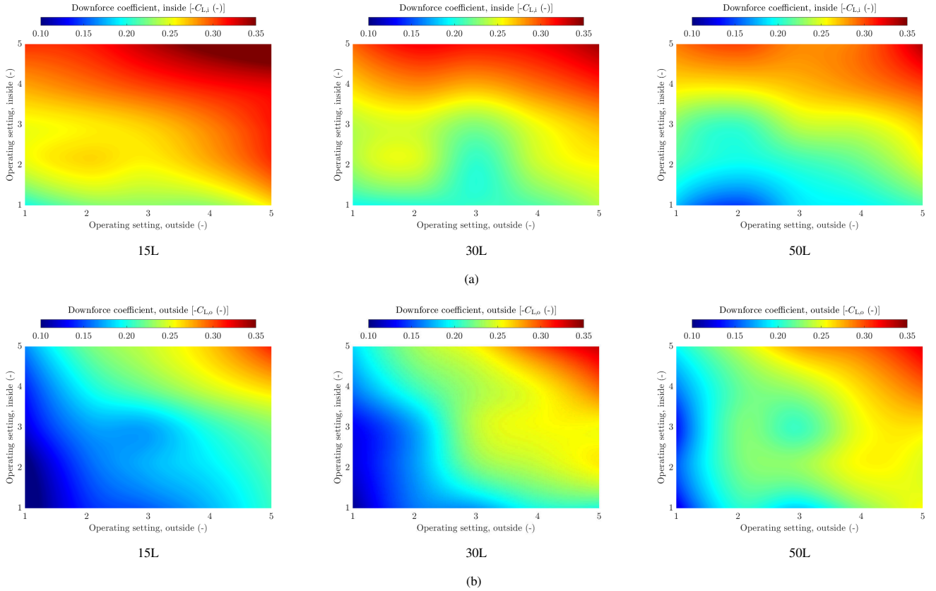
Figure 18: Downforce coefficients on the (a) inside tyres and (b) outside tyres as a function of the operating settings for the inside and outside located active aerodynamic devices of the split rear wing high-performance vehicle concept in various cornering conditions
