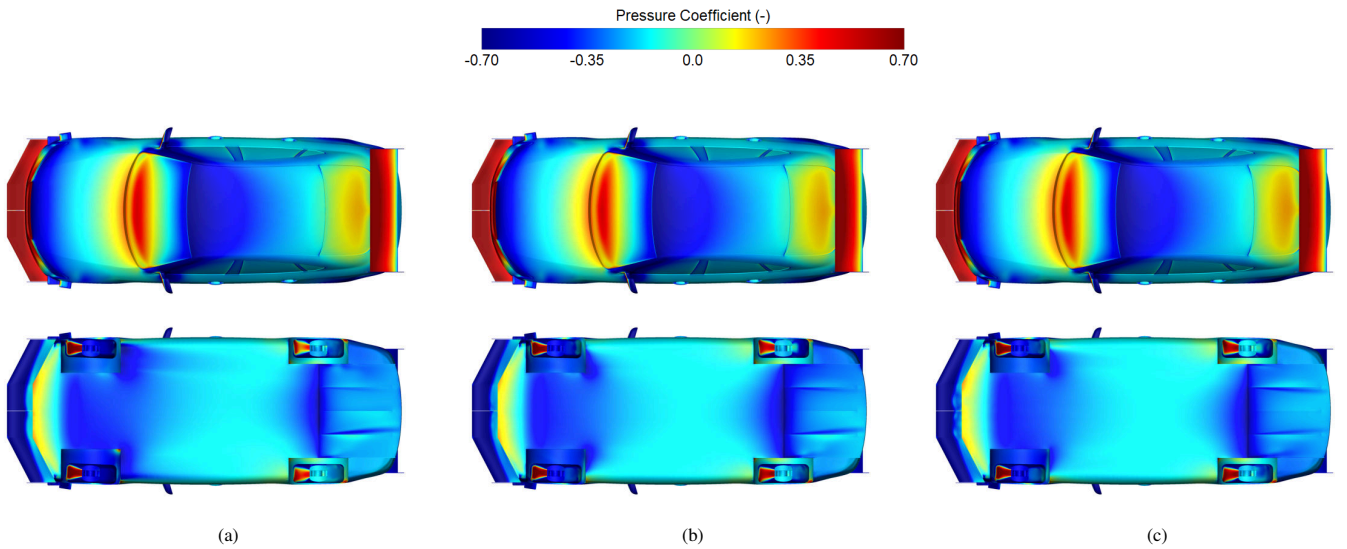
Figure 23: Pressure coefficient distribution on the tilted rear wing high-performance vehicle concept in its maximum symmetric operating state (5,5) in the (a) 15L radius corner, (b) 30L radius corner, and (c) 50L radius corner
