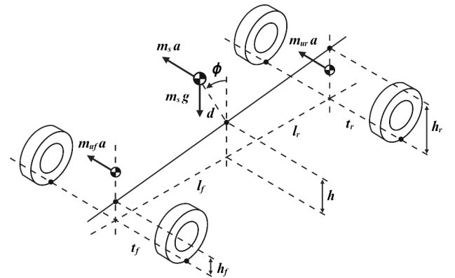
Figure 9: Schematic representation of lateral load transfer
