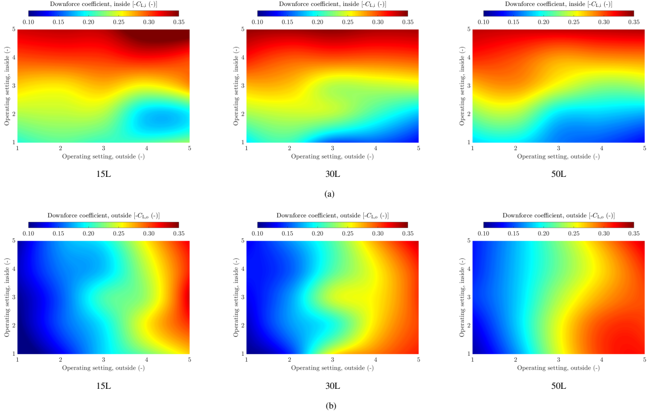
Figure 25: Downforce coefficients on the (a) inside tyres and (b) outside tyres as a function of the operating settings for the inside and outside located active aerodynamic devices of the tilted rear wing high-performance vehicle concept in various cornering conditions
