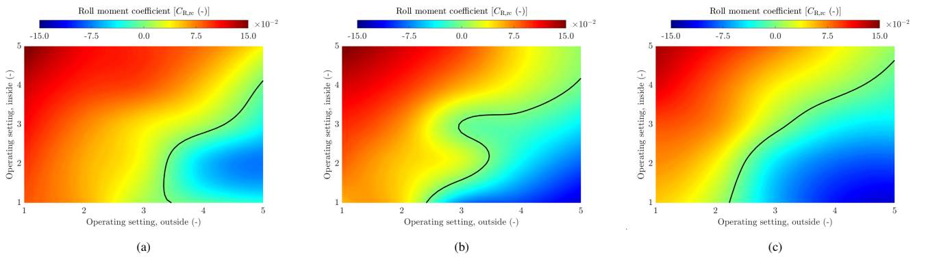
Figure 26: Aerodynamic roll moment coefficients about the vehicle's roll axis as a function of the operating settings for the inside and outside located active aerodynamic devices of the tilted rear wing high-performance vehicle concept in the (a) 15L radius corner, (b) 30L radius corner, and (c) 50L radius corner. The black contour lines mark an aerodynamic roll moment coefficient of zero.
