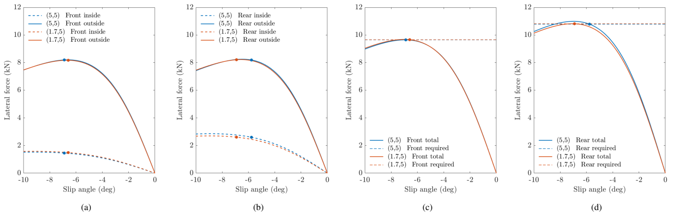
Figure 21: Comparison between the lateral forces produced by the (a) front tyres, (b) rear tyres, (c) front tyres combined, and (d) rear tyres combined of the split rear wing high-performance vehicle concept in its maximum symmetric (5,5) and optimal inside bias (1.7,5) operating states in the 50L radius corner
