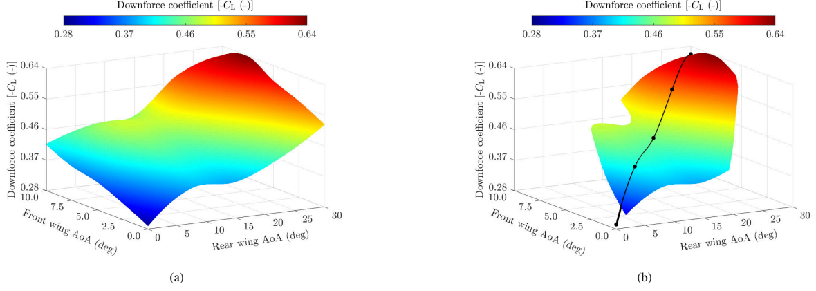
Figure 14: (a) Downforce coefficients on the vehicle body for the full range of simulated front and rear wing angles of attack, and (b) downforce coefficients on the vehicle body in the 40%-60% front axle downforce distribution region, including the determined operating line and settings utilised for the control strategy
