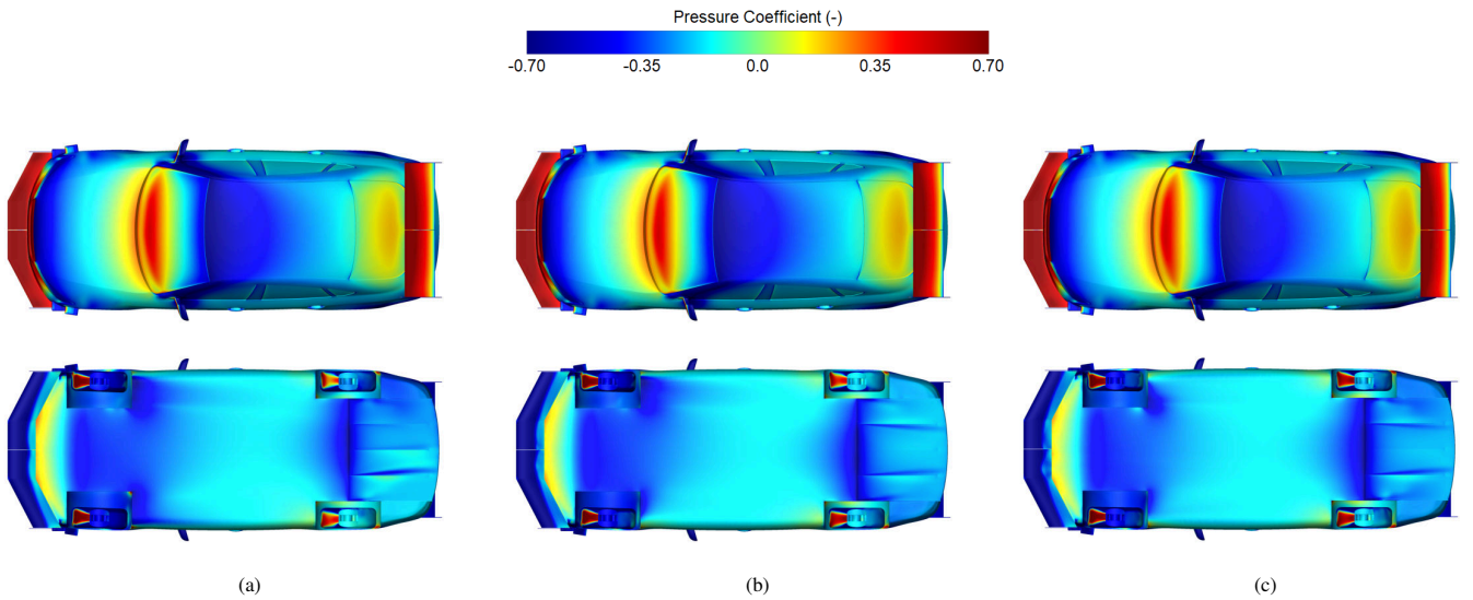
Figure 16: Pressure coefficient distribution on the split rear wing high-performance vehicle concept in its maximum symmetric operating state (5,5) in the (a) 15L radius corner, (b) 30L radius corner, and (c) 50L radius corner
