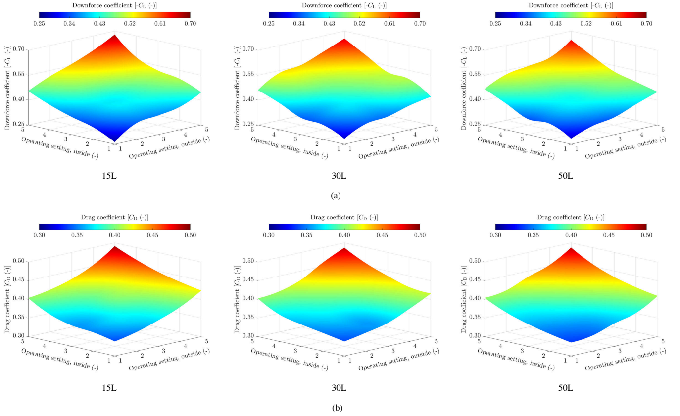
Figure 15: (a) Downforce coefficients and (b) drag coefficients as a function of the operating settings for the inside and outside located active aerodynamic devices of the split rear wing high-performance vehicle concept in various cornering conditions
