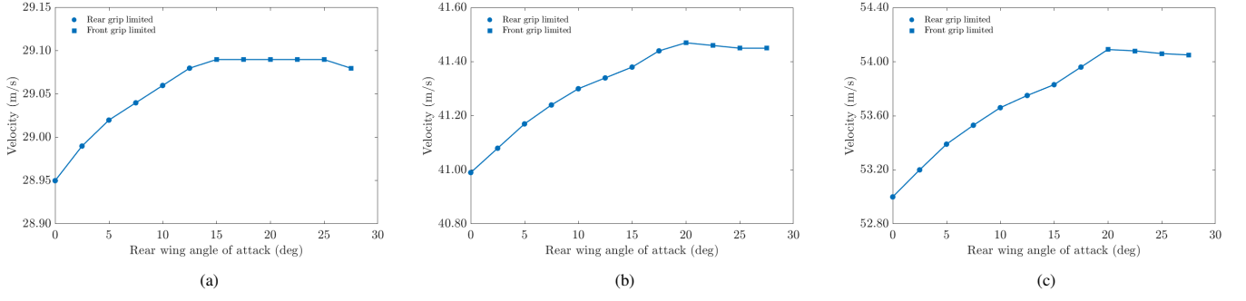
Figure 12: Maximum cornering velocity for the baseline DrivAer hp-F in the (a) 15L radius corner, (b) 30L radius corner, and (c) 50L radius corner operating conditions. The marker style indicates front or rear grip limit behaviour.
