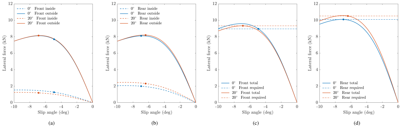
Figure 13: Comparison between the lateral forces produced by the (a) front tyres, (b) rear tyres, (c) front tyres combined, and (d) rear tyres combined of the baseline DrivAer hp-F with 0^\circ and 20^\circ rear wing angles of attack in the 50L radius corner
