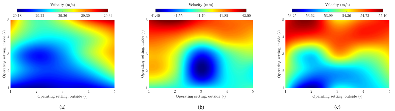
Figure 20: Maximum velocity as a function of the operating settings for the inside and outside located active aerodynamic devices of the split rear wing high-performance vehicle concept in the (a) 15L radius corner, (b) 30L radius corner, and (c) 50L radius corner
