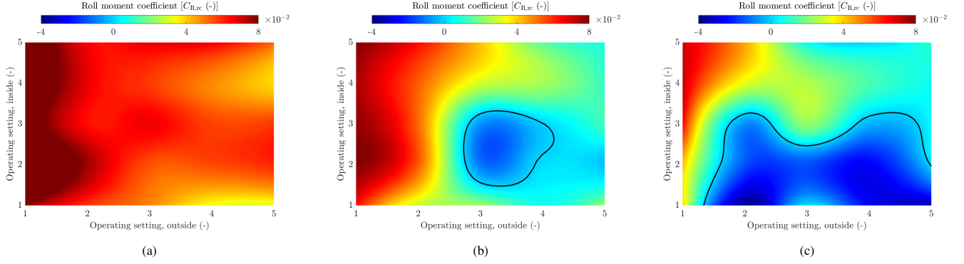
Figure 19: Aerodynamic roll moment coefficients about the vehicle's roll axis as a function of the operating settings for the inside and outside located active aerodynamic devices of the split rear wing high-performance vehicle concept in the (a) 15L radius corner, (b) 30L radius corner, and (c) 50L radius corner. The black contour lines mark an aerodynamic roll moment coefficient of zero.
