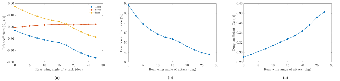
Figure 11: Wind tunnel measurement results of (a) lift coefficients, (b) downforce distribution, and (c) drag coefficients for the baseline DrivAer hp-F with varying rear wing angle of attack
