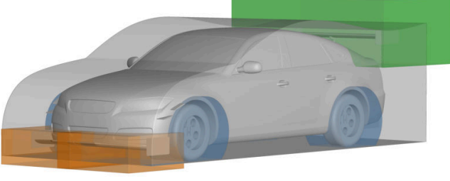
Figure 5: Overset interfaces of the component meshes
