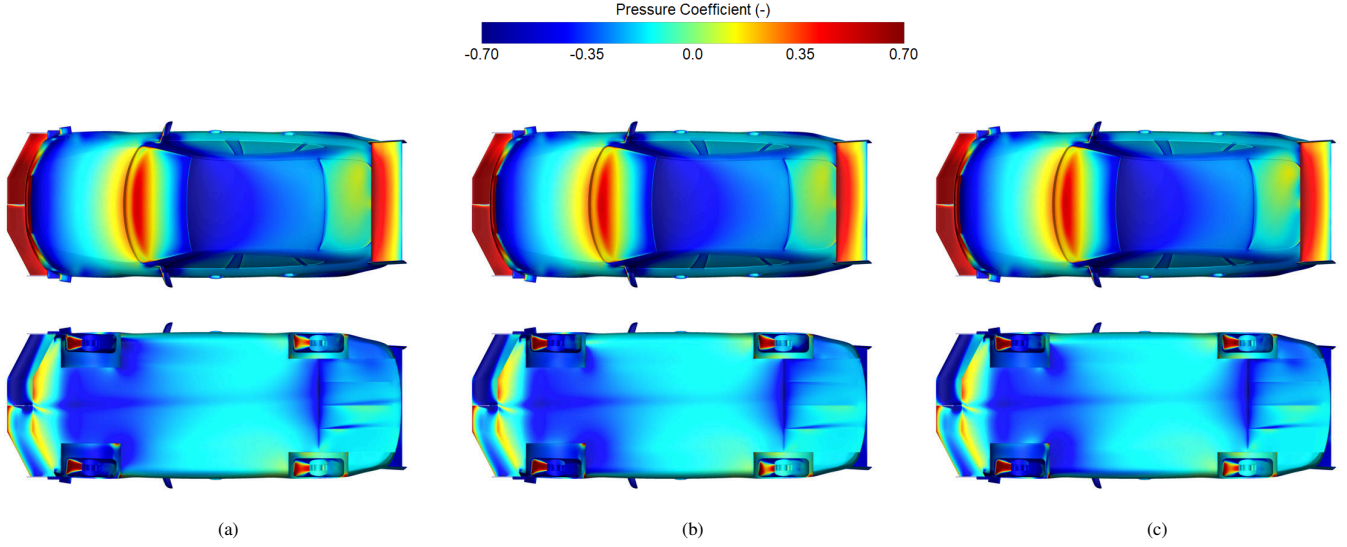
Figure 24: Pressure coefficient distribution on the tilted rear wing high-performance vehicle concept in its maximum inside bias operating state (1,5) in the (a) 15L radius corner, (b) 30L radius corner, and (c) 50L radius corner
