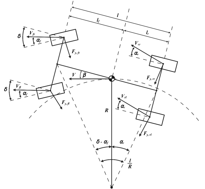
Figure 8: Schematic representation of the vehicle dynamics system
