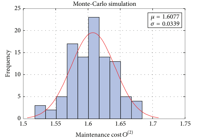
FIGURE 13: Monte-Carlo simulation results for maintenance cost O^{(2)} .
