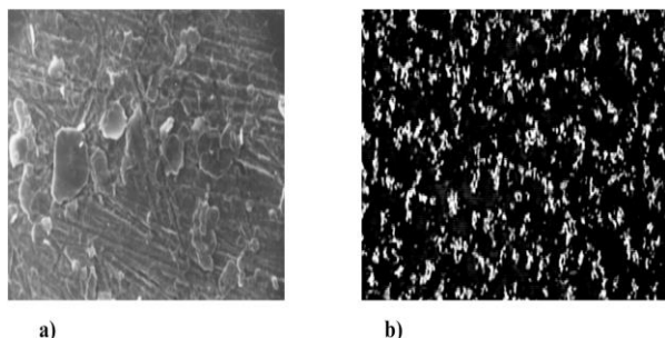
Figure 4. Photomicrograph of OSS-3 (a) before treatment, 20 \mu m and (b) after treatment, 20 \mu m (Sulaiman, et al. 2014:9)
