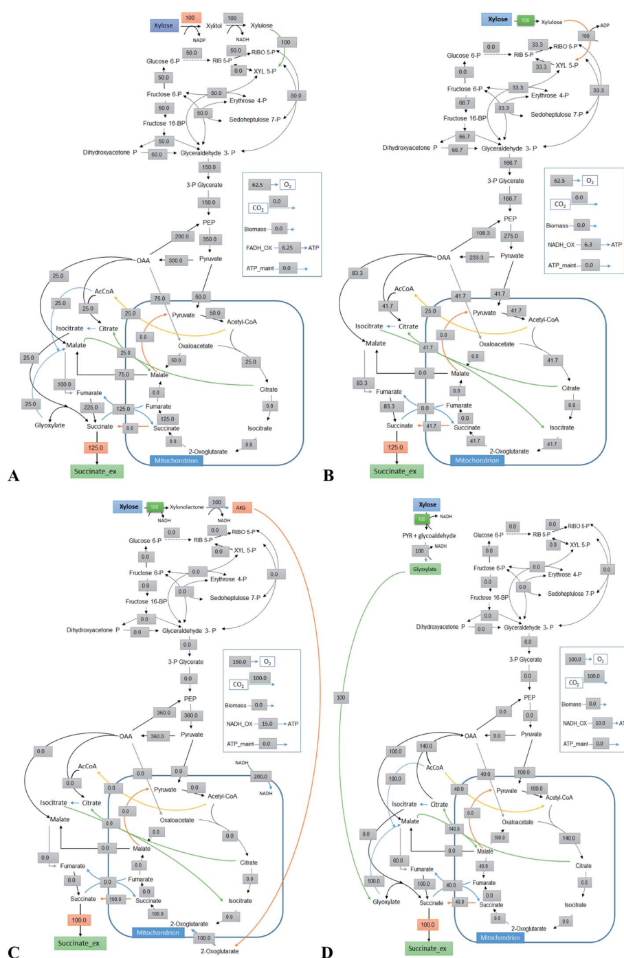
Fig. 10 Theoretical maximum (optimal) production of SA via (A) the XR-XDH pathway, (B) XI pathway, (C) XW pathway and (D) XD pathway in Y. lipolytica . Values normalised to 100% xylose uptake rate (mmol g -1 h -1 ).
