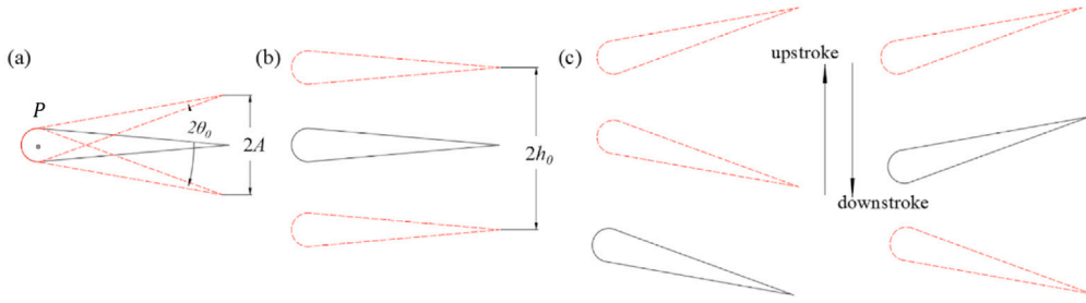
Fig. 3. The motions of foil: (a) pitching motion, (b) heaving motion and (c) flapping motion of a foil (Wu et al. [23]).
