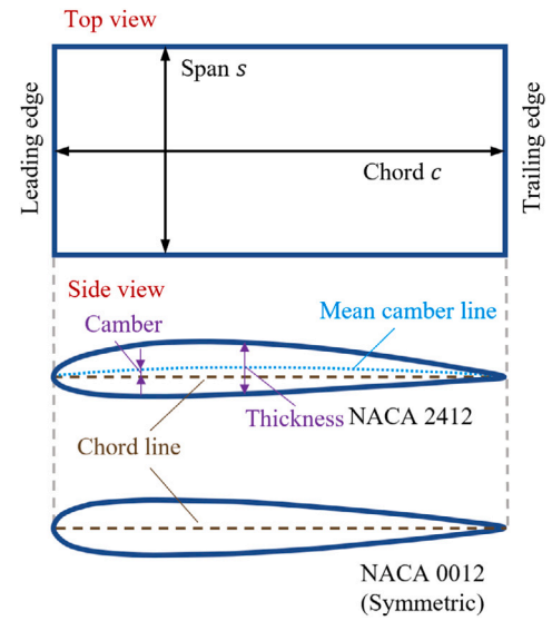
Fig. 2. The characteristics of the foil.
