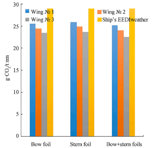
Fig. 9. Results EEDI weather of a container ship S-175 with wing devices at a representative sea condition (Ship speed = 22 kn) (Rozhdestvensky et al. [65]).
