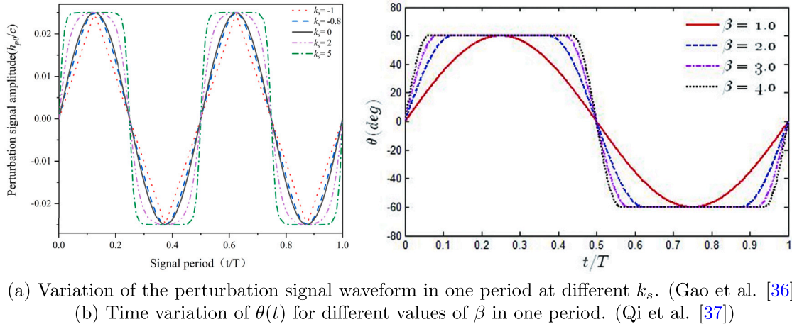
Fig. 5. Non-sinusoidal heaving and pitching motion signal.
