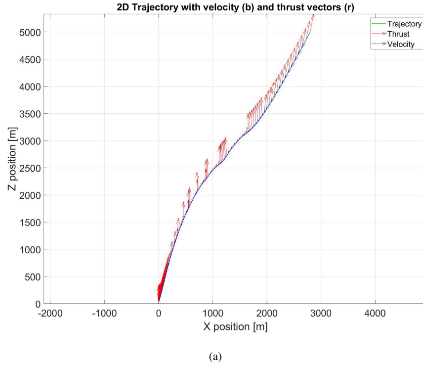
Figure 10: MPC: Landing trajectory with thrust vector.
