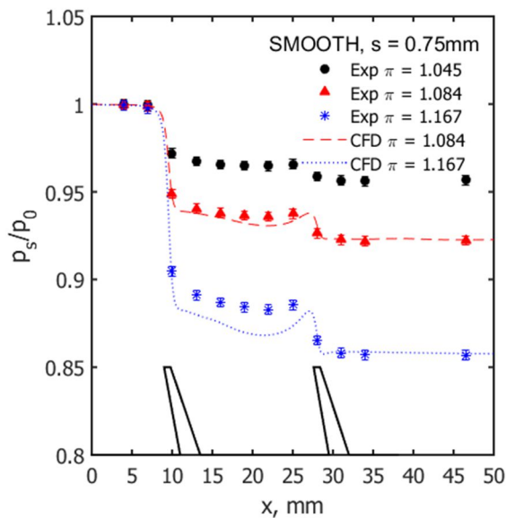
Figure 9. Static pressure distribution for smooth s = 0.75 mm, by low pressure ratios.
