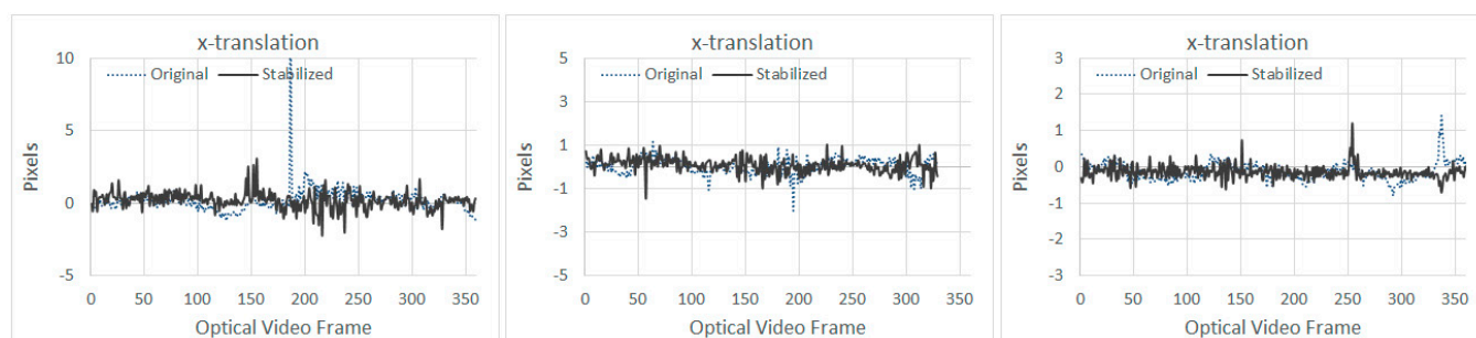
Figure 10. Results of x -translation at increasing UAV heights of 1.5, 2, and 3 m (from left to right) for SVR-LR, LR, and SVR-LR, respectively.
