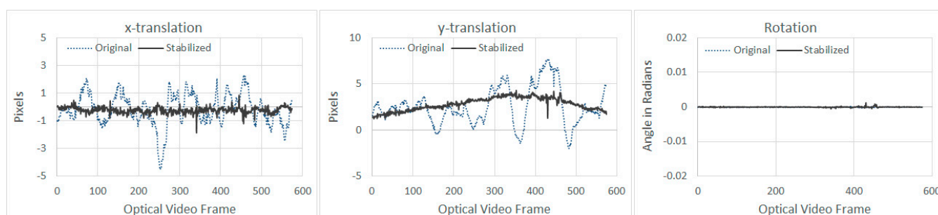
Figure 7. Comparison of extracted motion between original and stabilized frames for optical videos (result shown is that of GF-5s based smoothing).
