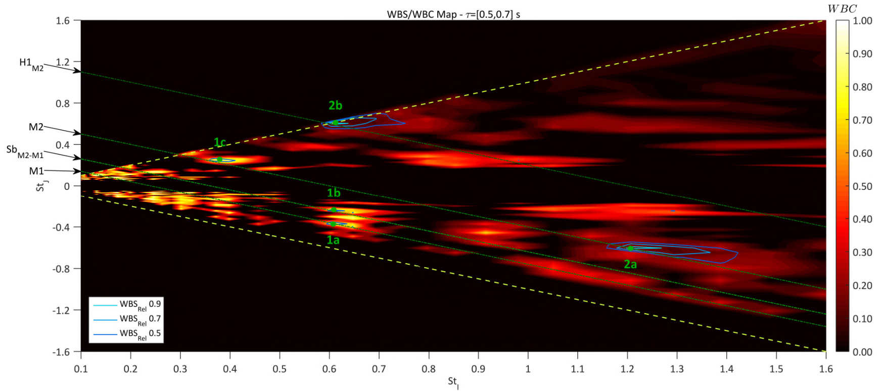
Figure 12. Wavelet auto-bi-spectrum and coherence of pressure signal at a cavity rear face, Mod002, x/L 1.0, 2y/W 0.0, z/D 0.0. The time of analysis was between 0.5 s and 0.7 s. Areas of high energy transfer are individuated by the super-imposition of WBS contours and WBC contours. Negative-constant-slope lines points which algebraic sum is constant.
