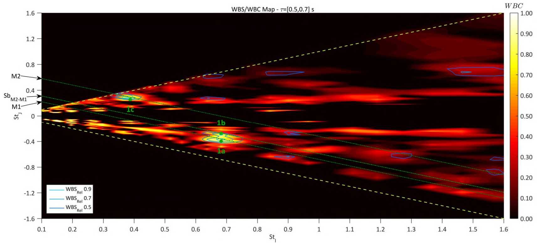
Figure 10. Wavelet auto-bi-spectrum and coherence of pressure signal at a cavity rear face, Mod000, x/L 1.0, 2y/W 0.0, z/D 0.0. The time of analysis was between 0.5 s and 0.7 s. Areas of high energy transfer are individuated by the super-imposition of WBS contours and WBC contours. Negative-constant-slope lines points which algebraic sum is constant.
