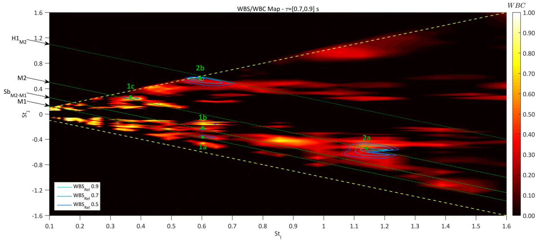
Figure 11. Wavelet auto-bi-spectrum and coherence of pressure signal at a cavity rear face, Mod001, x/L 1.0, 2y/W 0.0, z/D 0.0. The time of analysis was between 0.7 s and 0.9 s. Areas of high energy transfer are individuated by the super-imposition of WBS contours and WBC contours. Negative-constant-slope lines points which algebraic sum is constant.
