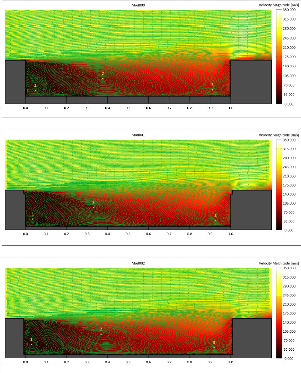
Figure 5. Mean velocity vector field at 2y/w = 0.0 coloured by velocity magnitude. Mod000 upper, Mod001 middle, Mod002 lower. The numbered points indicated the vortices centres. The impact point in the rear face of the shear layer streamlines indicates the maximum solicited area from an acoustic point of view. Flow from left to right.
