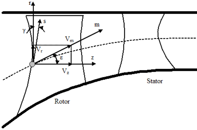
Fig. 1: Meridional plane vector – angle definition.
