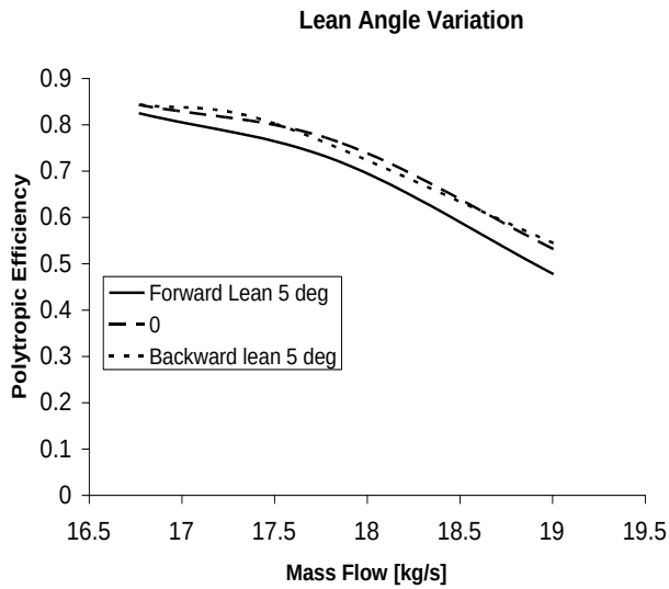
Fig. 13: The Compressor characteristic – Polytopic Efficiency for lean angle variation.
