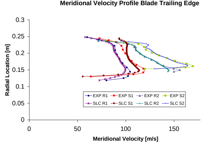
Fig. 8: Trailing edge meridional velocity profiles comparison between experimental data and in-viscid solver
