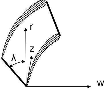
Fig. 6: Lean angle definition.
