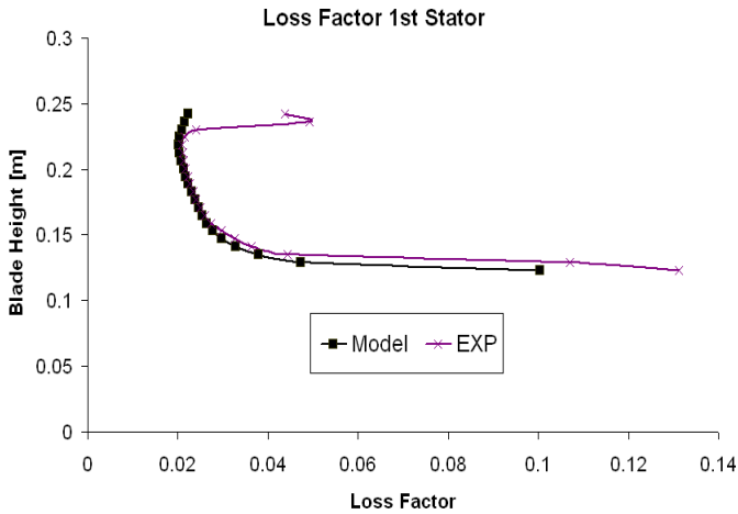
Fig. 11: Loss factor comparison – 1st stage stator
