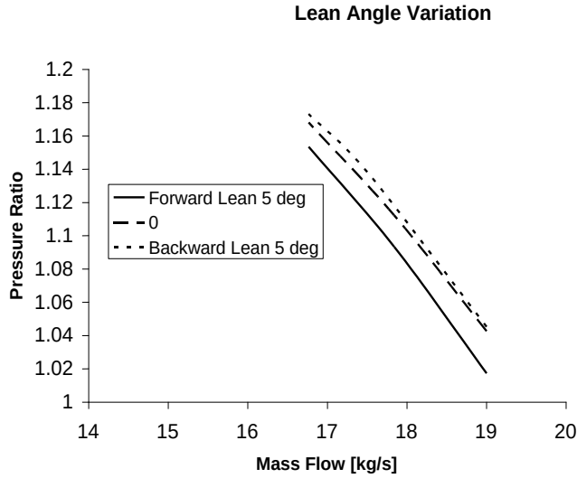
Fig. 12: Compressor characteristic – Pressure ratio for lean angle variation.
