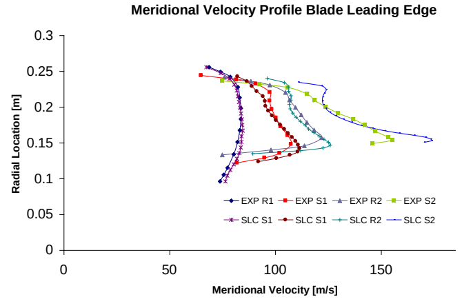
Fig. 9: Leading edge meridional velocity profiles comparison between experimental data and phenomenological module.
