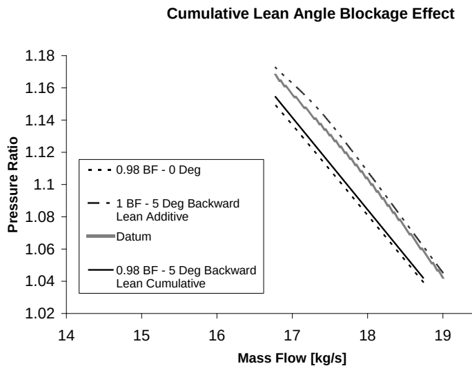
Fig. 16: Cumulative lean angle blockage effect on compressor performance.
