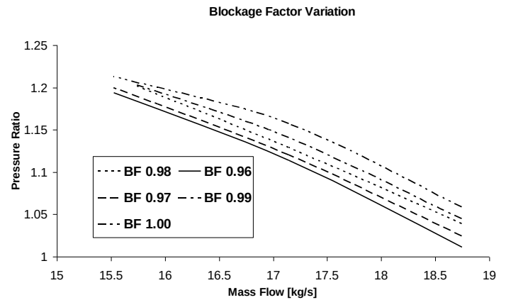
Fig. 14: Compressor characteristic – Pressure ratio for blockage factor variation.
