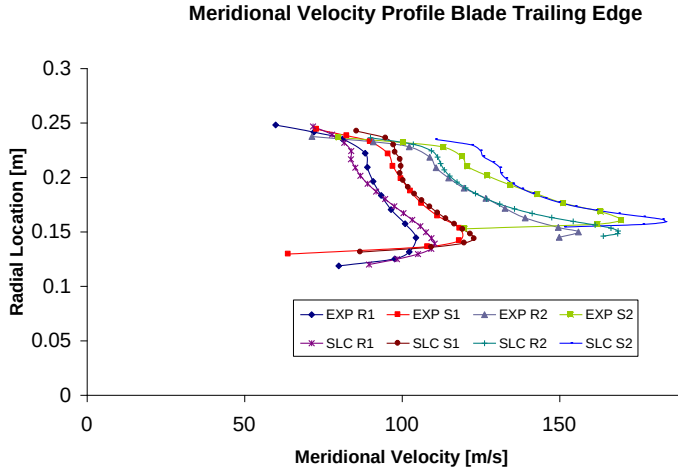
Fig. 10: The trailing edge meridional velocity profiles comparison between experimental data and phenomenological module
