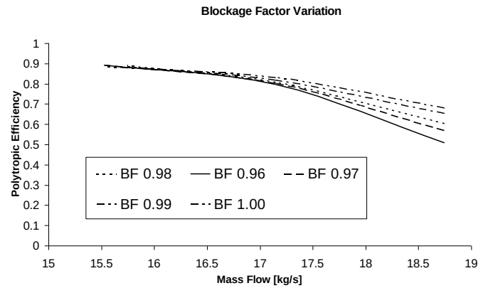
Fig. 15: The Compressor characteristic – Polytopic Efficiency for blockage factor variation.
