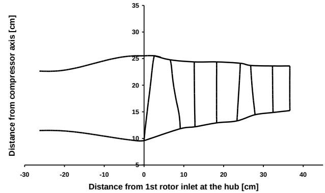
Fig. 4: Intake Compressor geometry.
