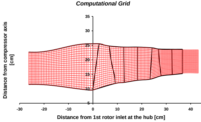
Fig. 5: Intake - Compressor geometry grid.
