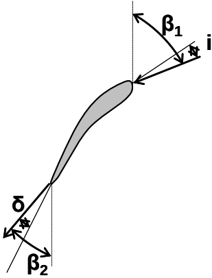
Fig. 2: Blade angle definition.
