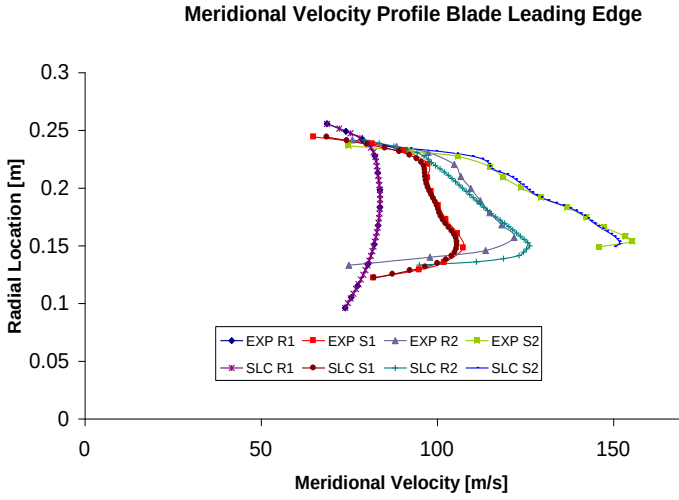
Fig. 7: Leading edge meridional velocity profiles comparison between experimental data and in-viscid solver
