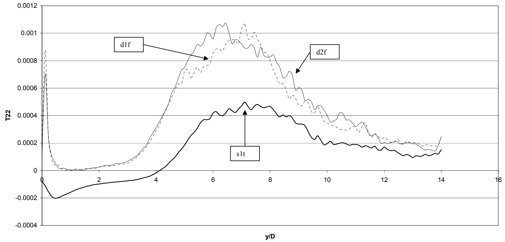
T22 Centrelines
