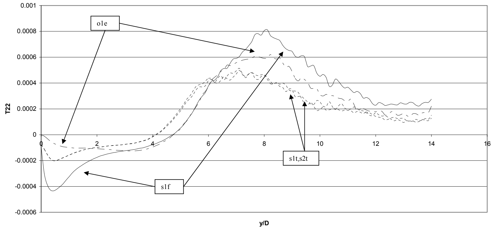
T22 Centrelines
