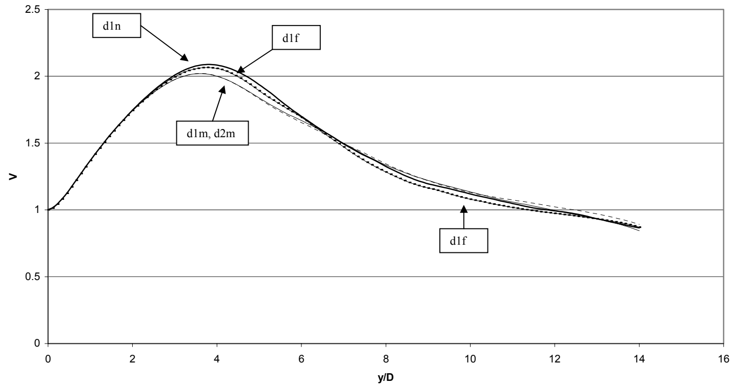
Velocity Centelines
