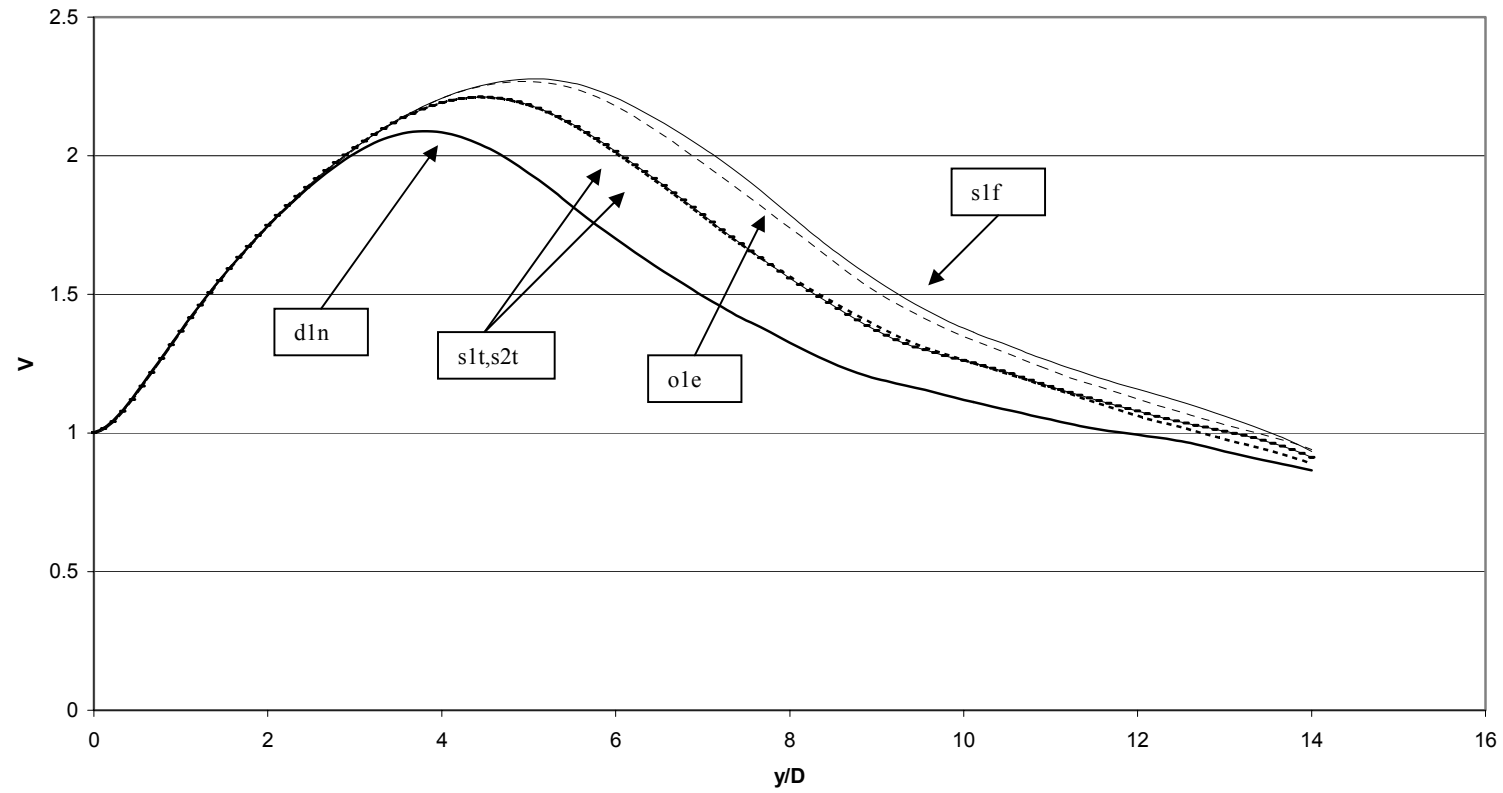
Velocity Centrelines
