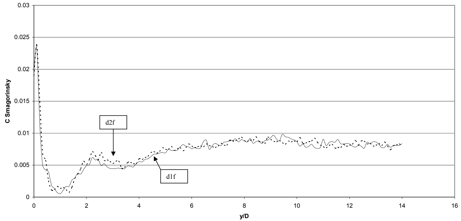
Smagorinsky Constant Centrelines
