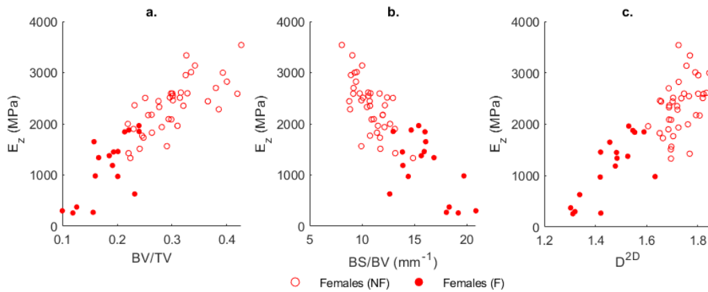
Figure 2: Relationships between a) BV/TV and E_z for non-fracture and fracture females, b) BS/BV and E_z for non-fracture and fracture females, c) D^{2D} and E_z for non-fracture and fracture females.
