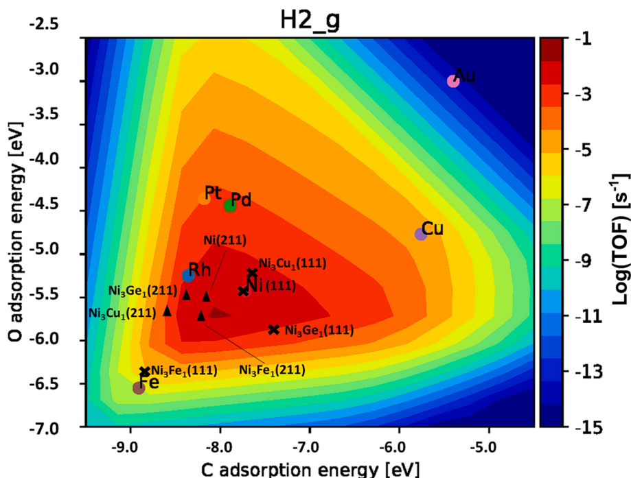
Fig. 9. TOF of H 2 production as a function of carbon and oxygen adsorption energies.
