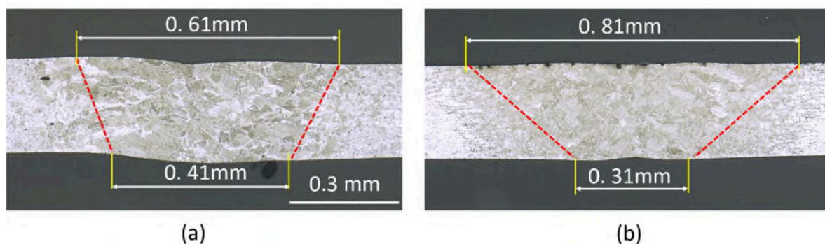
Figure 5. Welding samples of cold-rolled SPCD steel with a thickness of 0.25 mm were produced by (a) the novel GTAW torch and (b) the conventional GTAW torch.
