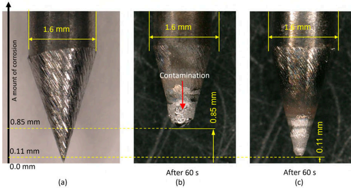
Figure 9. The tungsten electrode situation: (a) before welding, (b) after continuous welding 60 s with the conventional GTAW torch and (c) after continuous welding 60 s with the novel GTAW torch.
