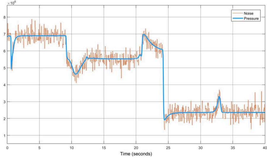
Fig. 5 Comparison of signal without and with noise injection in pump pressure.
