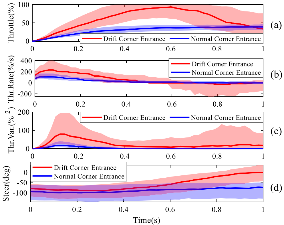
Figure 5. Driver inputs comparison (median value and interquartile range) between Drift Corner Entrance (DCE) and Normal Corner Entrance (NCE), for Intention to Start Drifting (ISD) recognition.
