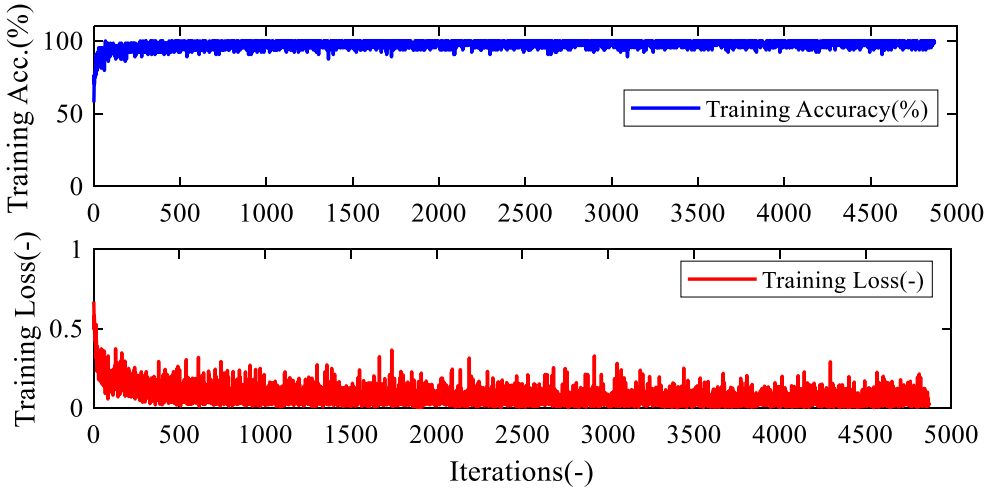
Figure 10. Bi-LSTM training progress for Intention to Start Drifting (ISD) recognition.
