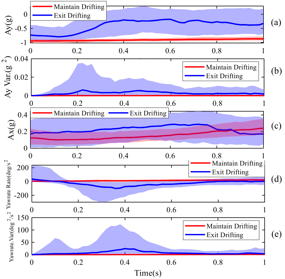
Figure 8. Vehicle acceleration signals comparison (median value and interquartile range) between MD and ED, for Intention to Exit Drifting (IED) recognition.
