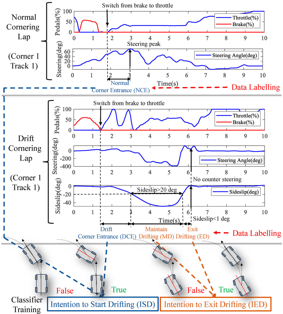
Figure 3. Labelling of data to classify two concerned intentions (ISD and IED).
