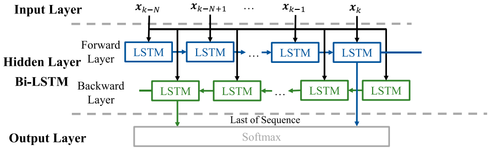
Figure 9. Structure of the Bi-LSTM.
