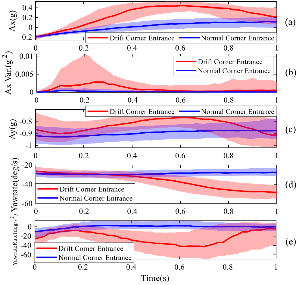
Figure 7. Vehicle acceleration signals comparison (median value and interquartile range) between Drift Corner Entrance (DCE) and Normal Corner Entrance (NCE), for Intention to Start Drifting (ISD) recognition.
