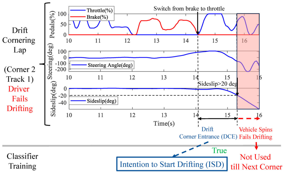
Figure 4. Labelling of data when the driver fails in drifting.
