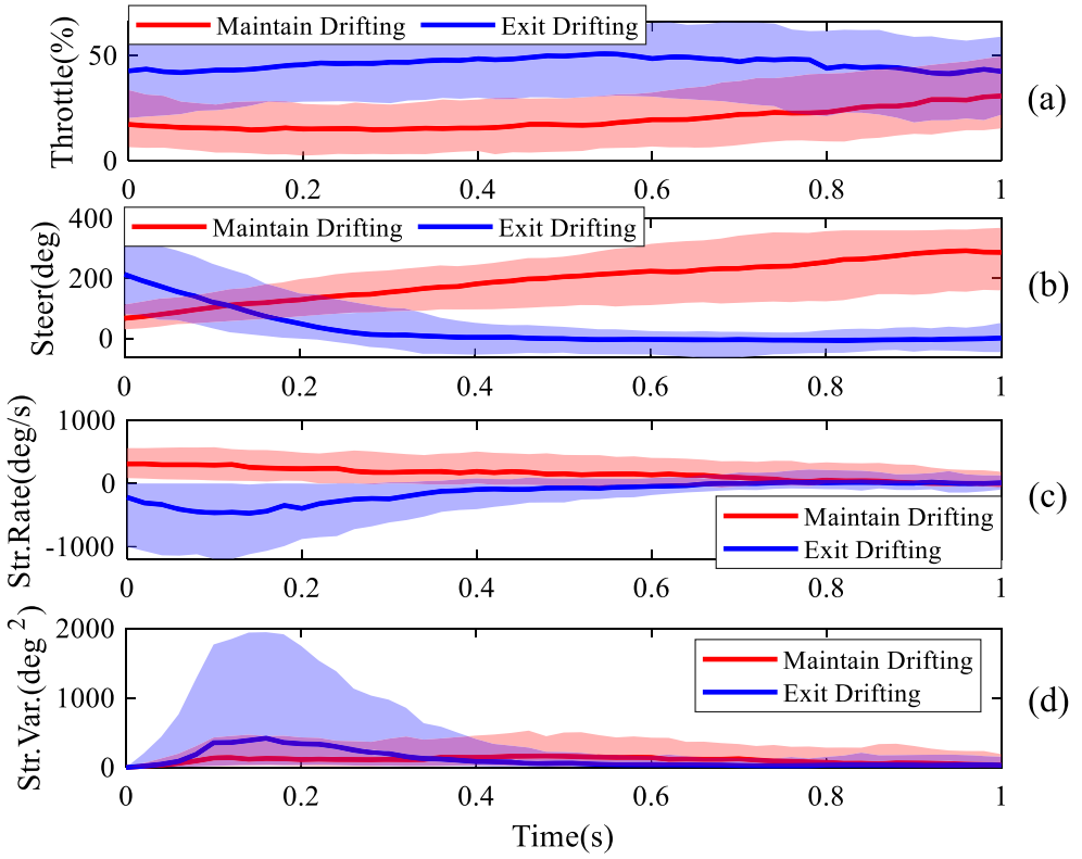
Figure 6. Driver inputs comparison (median value and interquartile range) between Maintain Drifting (MD) and Exit Drifting (ED), for Intention to Exit Drifting (IED) recognition.
