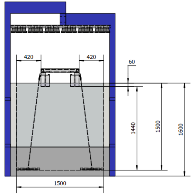
FIGURE 4: Section view of the solar+wave experimental facility; dimensions in mm
