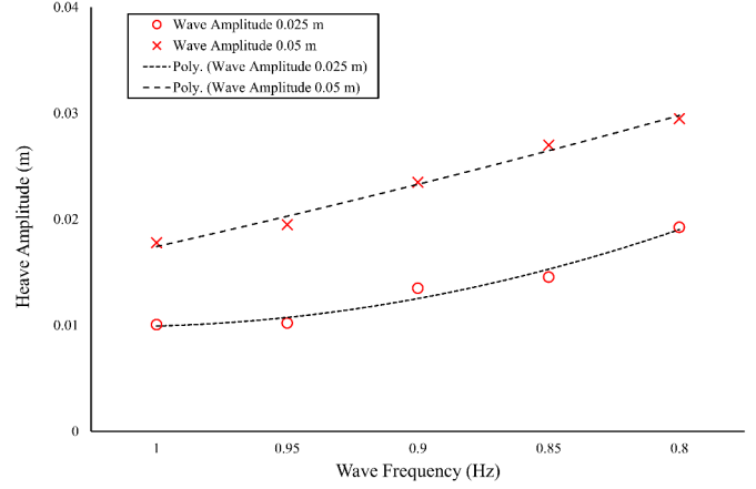
FIGURE 12: Heave amplitude of the structure in waves
