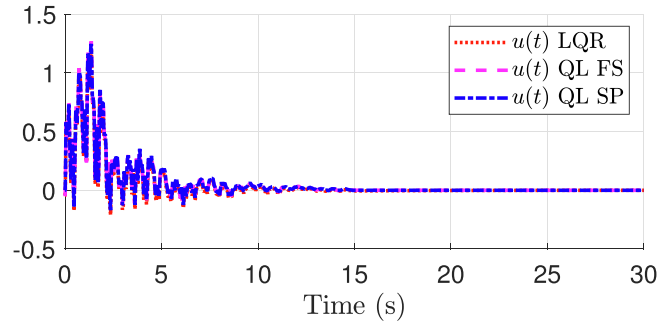
Fig. 3. Control input comparison.
