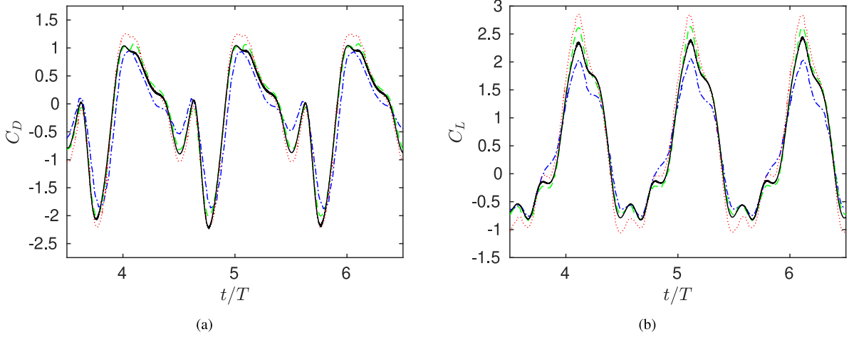
Fig. 13. Temporal evolution of the drag C_D (a) and lift C_L (b) coefficients for the flow over a flapping ellipse at Re = 157 : (—) present results, (·····) immersed boundary method of [15], (---) immersed boundary method of [34], (- · - ·) body-conformal mesh method [35].
