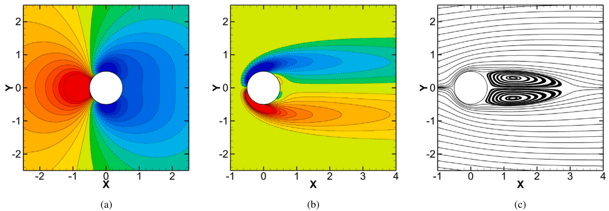
Fig. 7. Instantaneous pressure contours (a), vorticity contours (b), and streamlines (c) for the flow over a stationary cylinder at Re = 40 . Where the pressure contours are varied from -0.3 (blue) to 0.3 (red) and the vorticity contours are varied from -3 (blue) to 3 (red).
