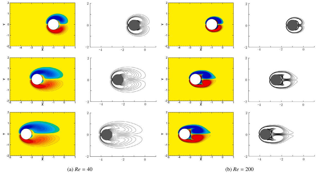
Fig. 11. Instantaneous vorticity contours at three different time instances t = 1 (top), 2.5 (middle), and 3.5 (bottom) for the flow over an impulsively started cylinder at Re = 40 (a) and Re = 200 (b). The present results correspond to the colored contours and the results acquired by [13] correspond to the black/white contours. The present vorticity contours are varied from -3 (blue) to 3 (red).
