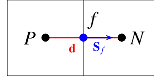
Fig. 2. Face area normal vector \mathbf{S}_f for Cartesian uniform meshes.
