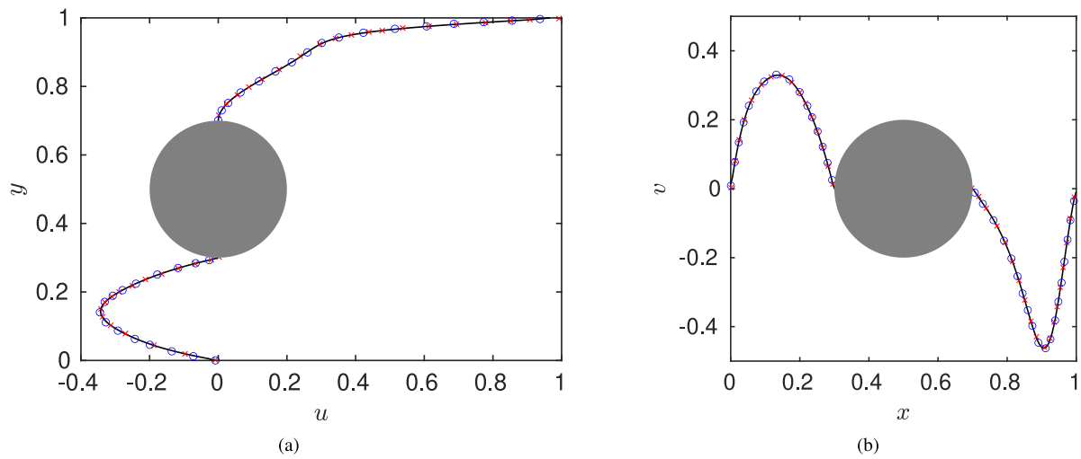
Fig. 6. Velocity u component along x = 0.5 (a) and velocity v components along y = 0.5 (b) for the lid-driven cavity with the embedded cylinder at Re = 1000 . Solid lines (—) correspond to the present results, (O) symbols correspond to the data reported in [23], and (x) symbols correspond to the data reported in [15].
