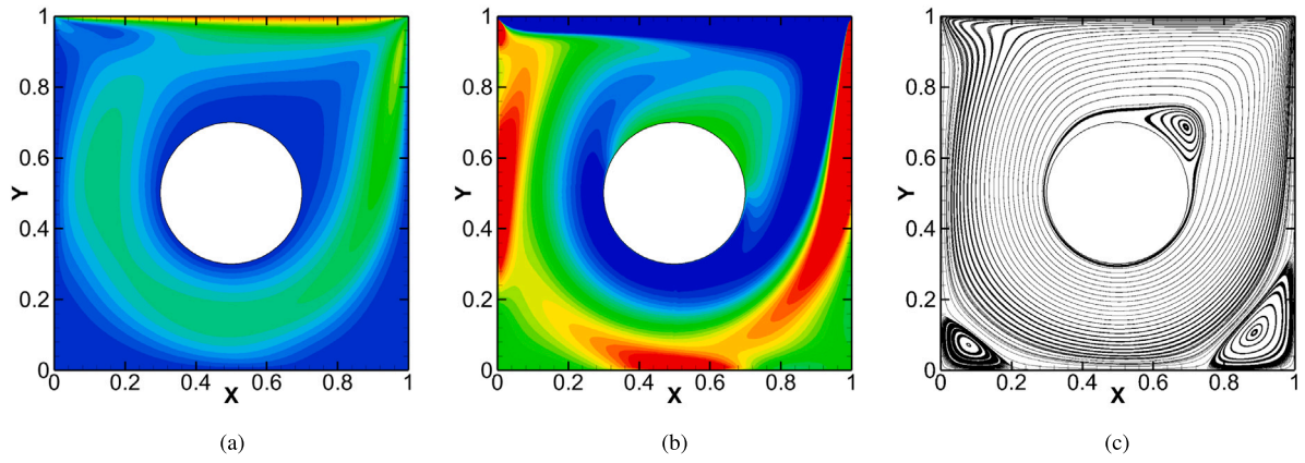
Fig. 5. Velocity magnitude contours (a), vorticity contours (b), and streamlines (c) for the lid-driven cavity with the embedded cylinder at Re = 1000 . Where the velocity magnitude contours are varied from 0 (blue) to 1 (red) and the vorticity contours are varied from -3 (blue) to 3 (red).
