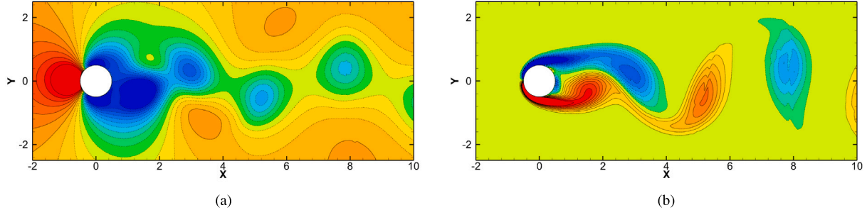
Fig. 8. Instantaneous pressure contours (a) and vorticity (b) contours for the flow over a stationary cylinder at Re = 100 . Where the pressure contours are varied from -0.4 (blue) to 0.3 (red) and the vorticity contours are varied from -3 (blue) to 3 (red).
