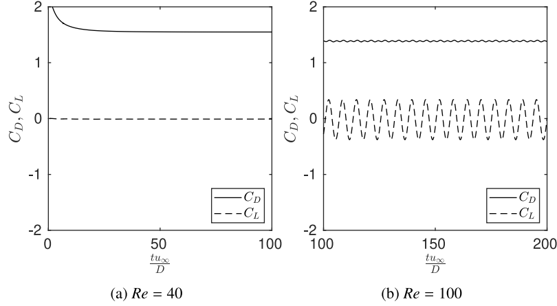
Fig. 9. Temporal evolution of the drag C_D and lift C_L coefficients for the flow over a stationary cylinder at different Re .
