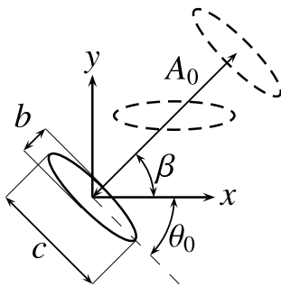
Fig. 12. Configuration of the flapping ellipse.
