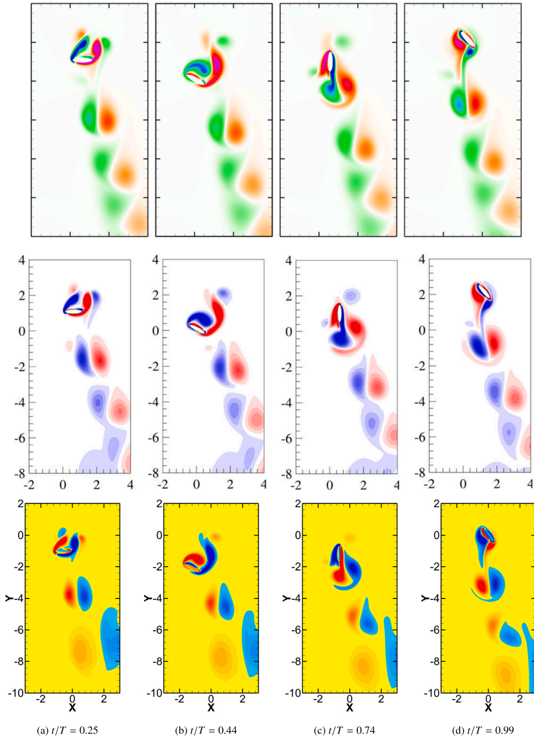
Fig. 14. Instantaneous vorticity contours at four different period instances t/T for the flow over a flapping ellipse at Re = 157 . The present results are placed at the bottom, the results corresponding to [15] are placed in the middle, and the results corresponding to [34] are placed at the top. The present vorticity contours are varied from -3 (blue) to 3 (red).
