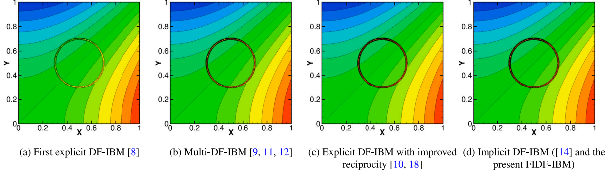
Fig. 3. Velocity ( u ) contours for different DF-IBM strategies. Where the vorticity contours are varied from -2 (blue) to 0 (red).
