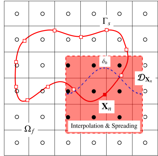
Fig. 1. Interpolation and spreading operators with the help of a smoothed approximation of the Dirac delta function in the DF-IBM.
