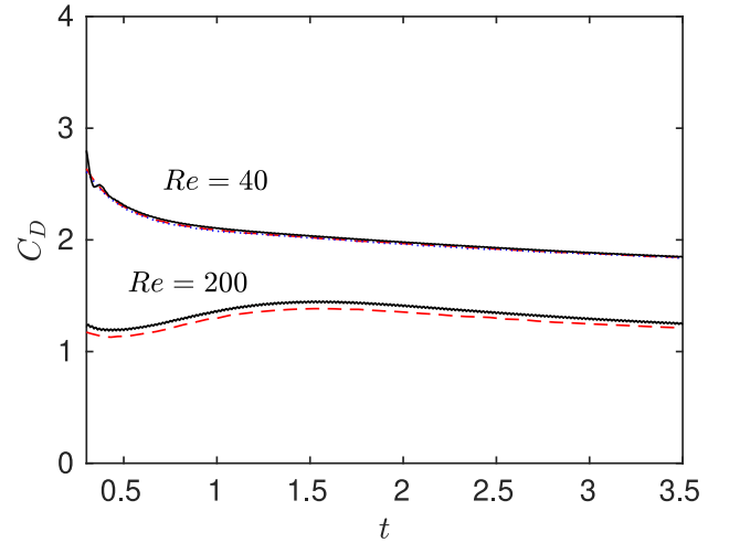
Fig. 10. Temporal evolution of the drag C_D coefficient for the flow over an impulsively started cylinder at Re = 40 and Re = 200 : (—) present results, (·····) data reported in [15], (---) data reported in [13].
