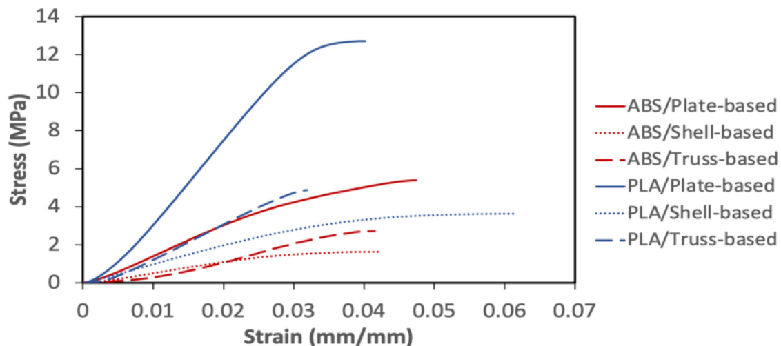
Figure 15. The stress–strain curve provides the mechanical behaviour of the samples and could help to find a microstructural design and properties [113].
