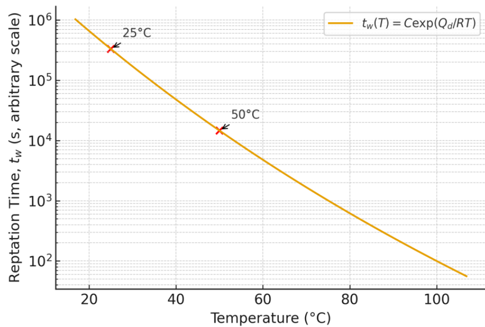
Figure 8. Schematic of the Arrhenius dependence of reptation time, t_w(T) = C \cdot e^{(Q_d/RT)} . A modest increase in chamber temperature (25 °C \rightarrow 50 °C) exponentially reduces t_w , enabling greater chain mobility and interdiffusion.
