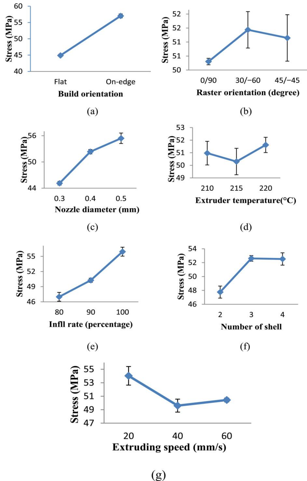
Figure 10. Stress–strain responses corresponding to each parameter. (a) shows the effect of build orientation, (b) shows the effect of raster orientation, (c) shows the effect of nozzle diameter, (d) shows the effect of extruder temperature, (e) shows the effect of infill rate, (f) shows the effect of number of shells, and (g) shows the effect of extruding speed [67].
