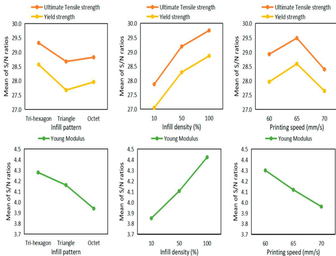
Figure 12. (S/N) ratio analysis of ABS specimens under tensile loading [87].
