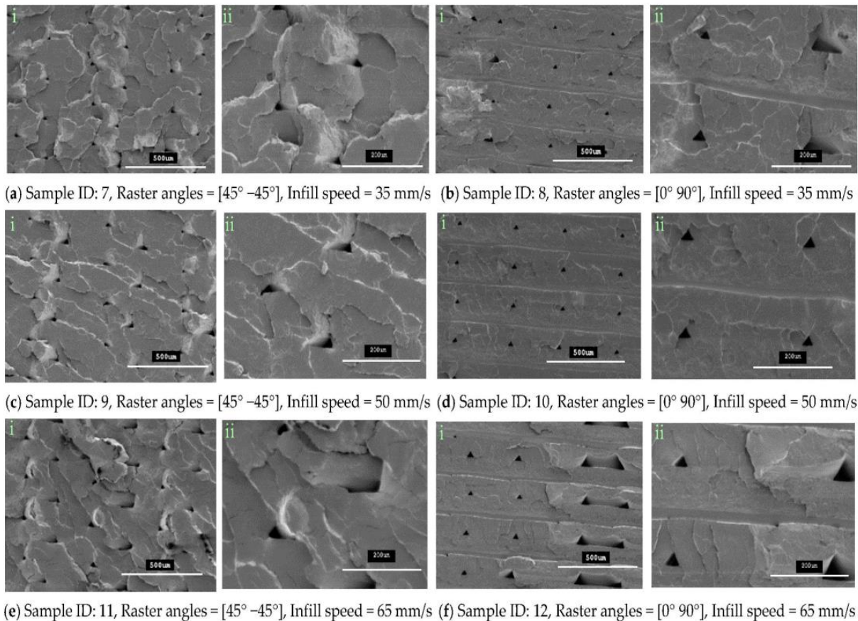
Figure 3. SEM micrographs of tensile-fractured specimens printed at different raster angles and infill speeds. Panels (i) were imaged at \sim 500\times magnification (scale bar = 500 \mu\text{m} ), and panels (ii) at \sim 800\times magnification (scale bar = 200 \mu\text{m} ) [19].
