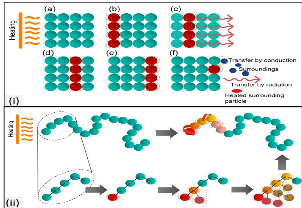
Figure 4. (i) How heat transfer occurs inside the crystalline polymer particles, where (a) represents the ideal order of the polymer lattices that start receiving heat. (b–e) illustrate efficient heat transfer within a perfectly arranged lattice structure, where thermal energy is sequentially conducted from one lattice element to the next. At stage (f), the outermost lattice at the polymer surface transfers heat by conduction when in contact with a solid surface, and by convection and radiation to the surrounding ambient environment.; (ii) how heat transfer occurs inside the amorphous polymer particles. The green circular regions represent amorphous polymer particles at room temperature. Upon heat input, these regions initially turn red, indicating the highest local temperature. As heat is transferred randomly through the amorphous polymer structure, a thermal gradient develops between neighbouring particles, which is visually represented by a gradual colour transition from red to yellow, where yellow denotes the lowest temperature prior to returning to room temperature [11].
