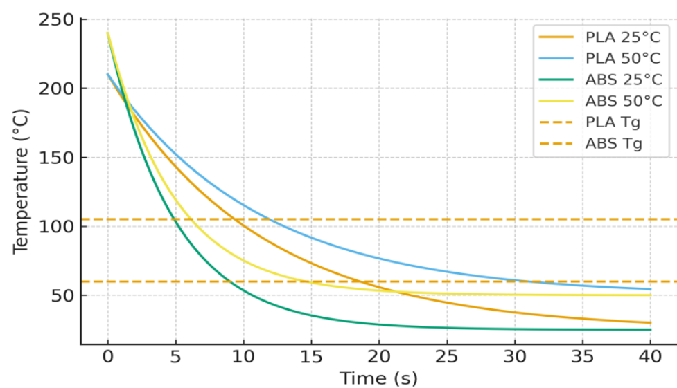
Figure 6. Cooling histories of PLA and ABS filaments predicted by the lumped-capacitance model under two ambient conditions.
