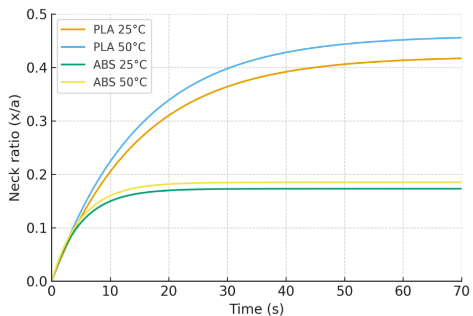
Figure 7. Evolution of the interfacial neck ratio ( x/a ) between adjacent roads.
