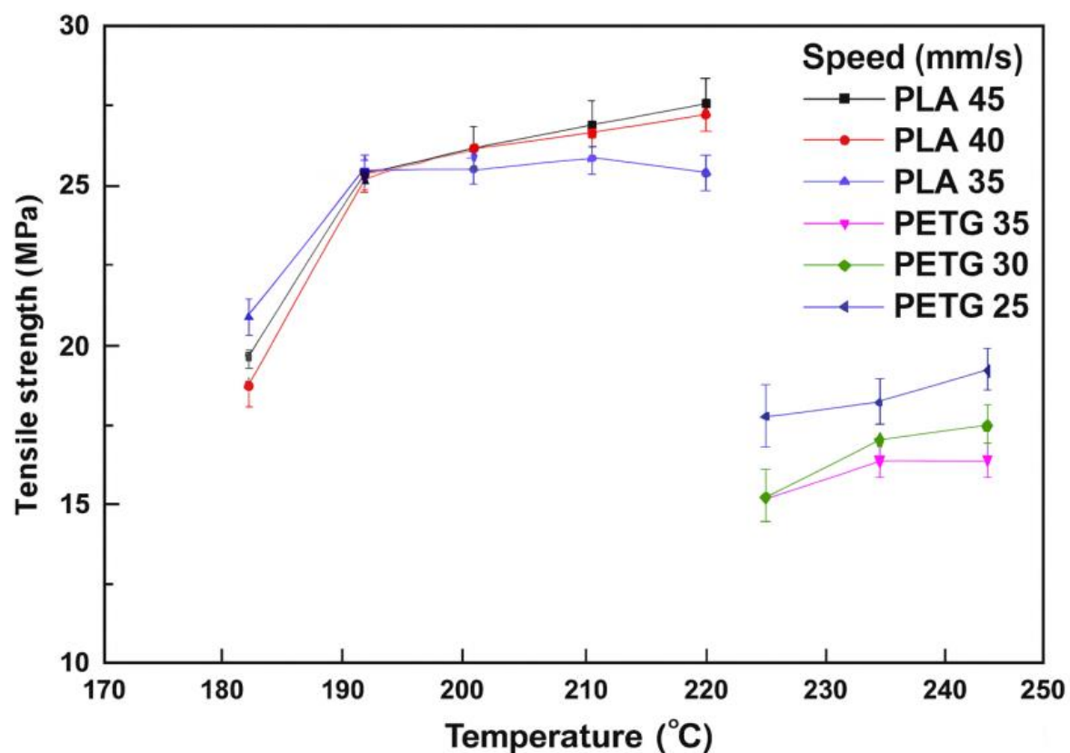
Figure 13. Effect of Nozzle Temperature on the Tensile Strength [95].
