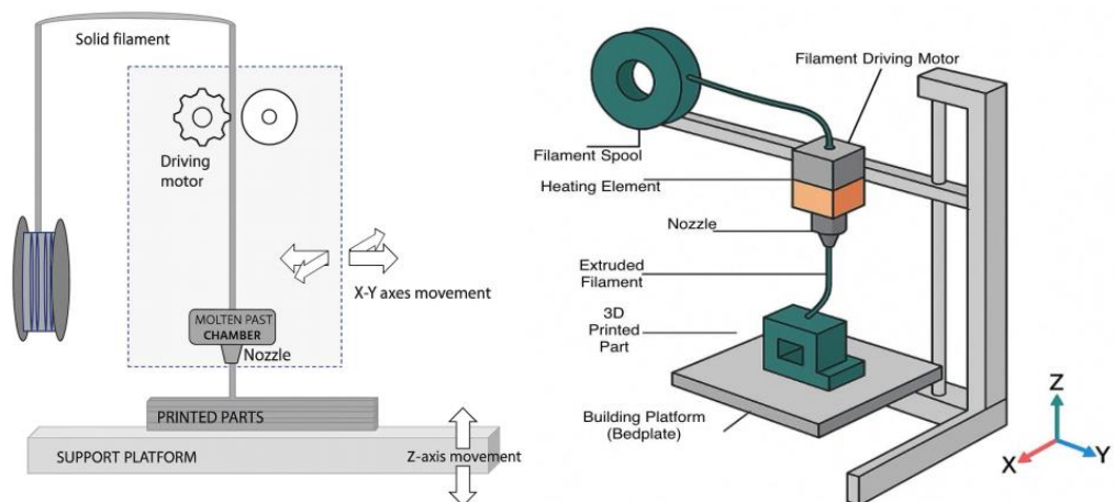
Figure 2. On the left, Schematic for FDM Process [10]; On the right, Parts of FDM Printer [14].
