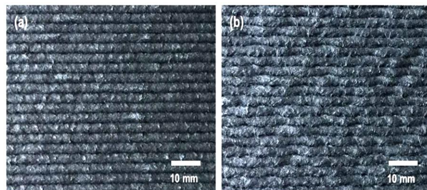
Figure 14. SEM images (a) show the effect of heating by IR on layers, and (b) No IR heating [102].
