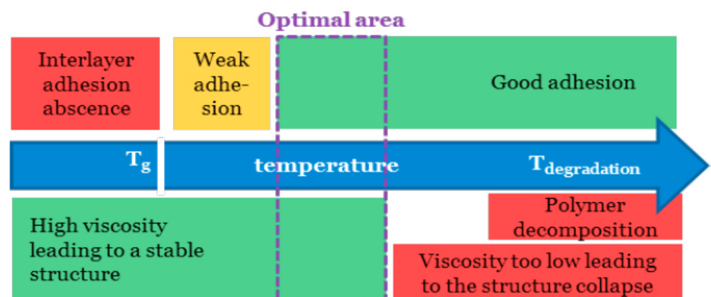
Figure 5. Optimal and non-optimal Nozzle temperature Effect on polymers [24].
