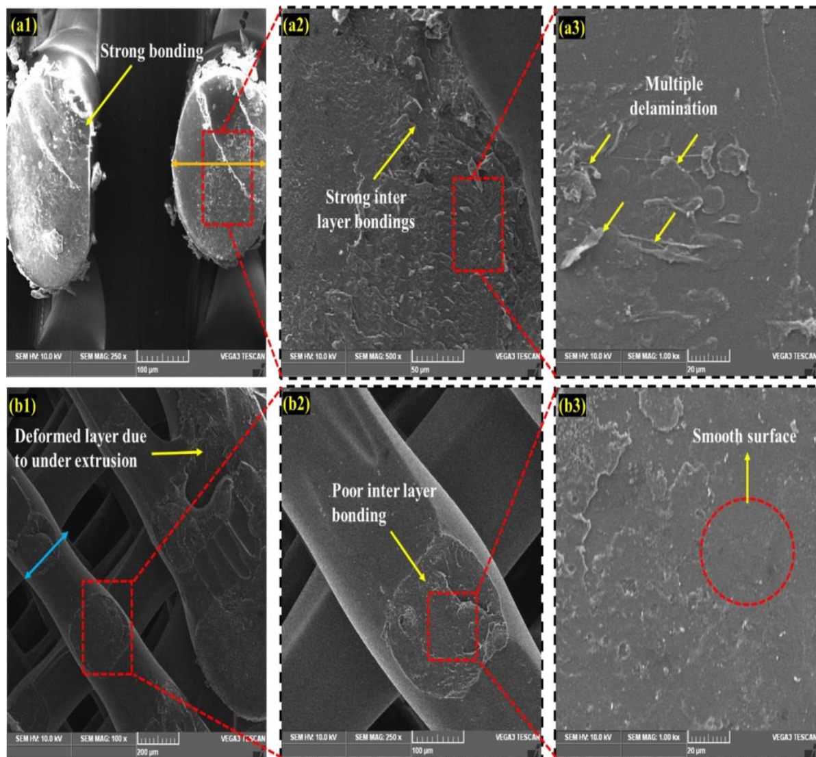
Figure 11. Comparison of fracture mechanism of tensile specimens (a1–a3), optimum parameters and (b1–b3) un-optimum parameters [70].
