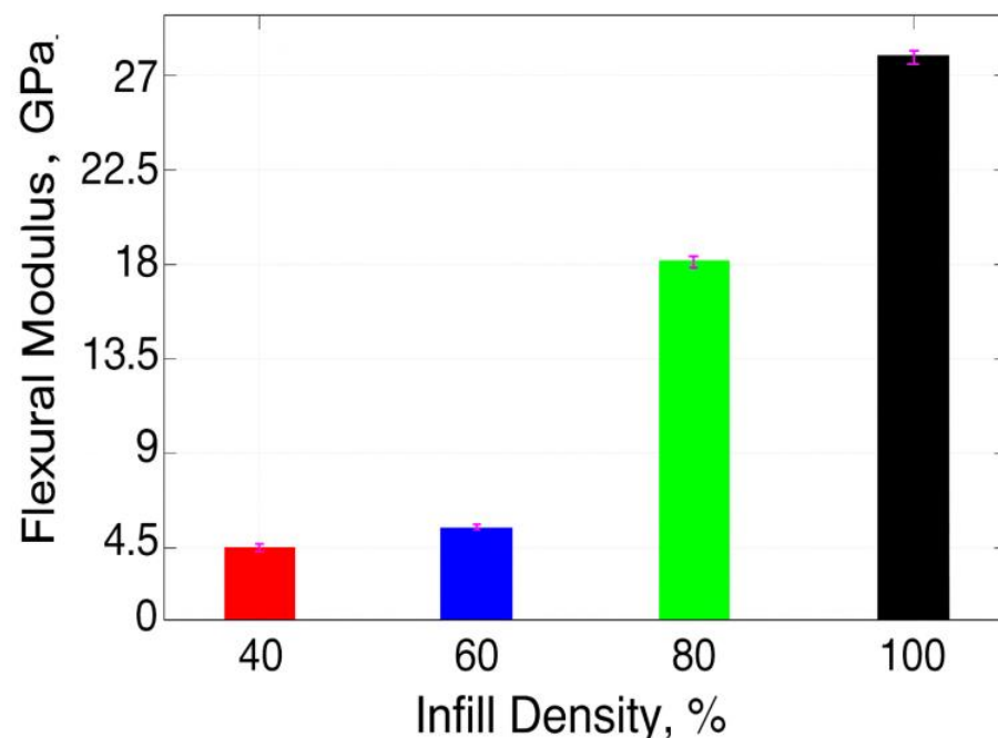
Figure 9. Influence of infill density on flexural modulus, The pink bars typically represent variability or uncertainty in the measured flexural modulus [63].
