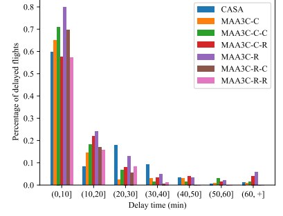
Fig. 10: Delay distribution of Case 4.
