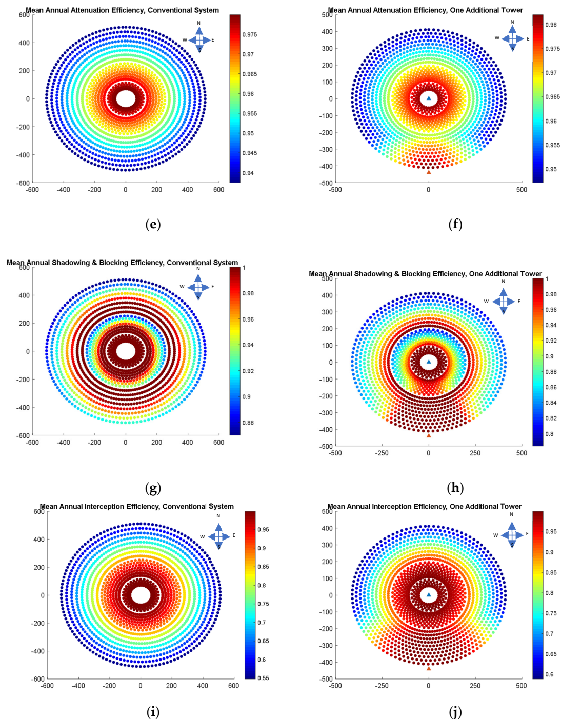
Figure 12. a, c, g, i) Conventional field: mean annual efficiency, cosine, attenuation, shadowing & blocking and interception efficiency respectively. b, d, f, h, j) Multi-tower field, one additional tower: mean annual efficiency, cosine, attenuation, shadowing and blocking and interception efficiency respectively.
