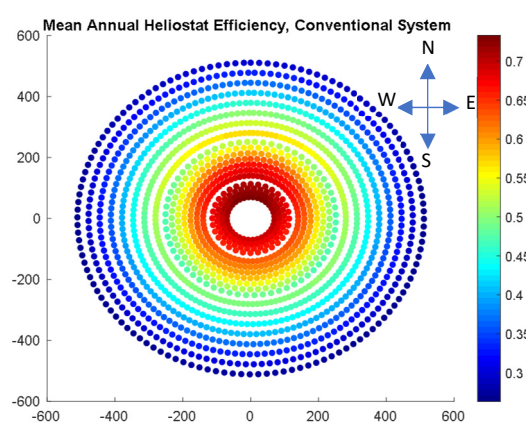
Figure 7. Field layout of a 50MWth Conventional Power Tower System.
