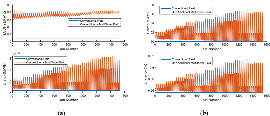
Figure 2 a) Levelized Cost of Heat (LCOH) and energy output with one additional multi-tower system b) thermal power and mean annual efficiency with one additional multi-tower system.
