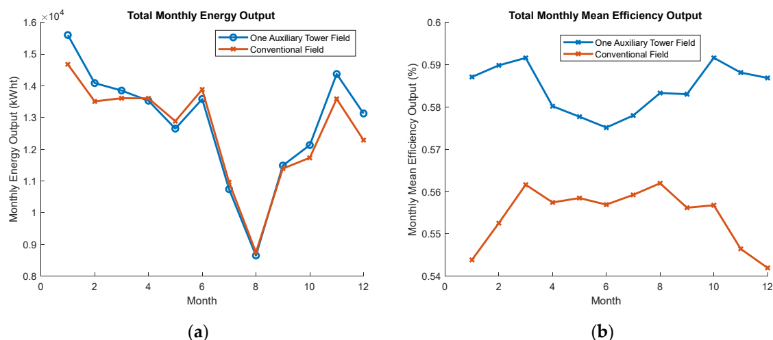
Figure 4 a) Total monthly energy output, conventional and one additional tower field; b) Total monthly mean efficiency output, conventional and one additional tower field.
