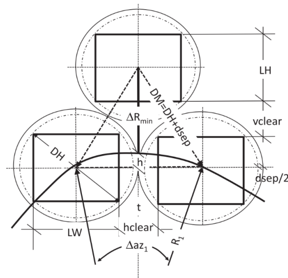
Figure 1. Parameters defining the layout of the field.
