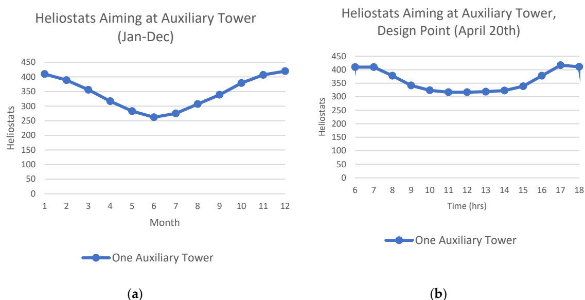
Figure 3 a) Heliostats aiming at the auxiliary tower through the year; b) Heliostats aiming at the auxiliary tower during sunshine hours at the design point date.
