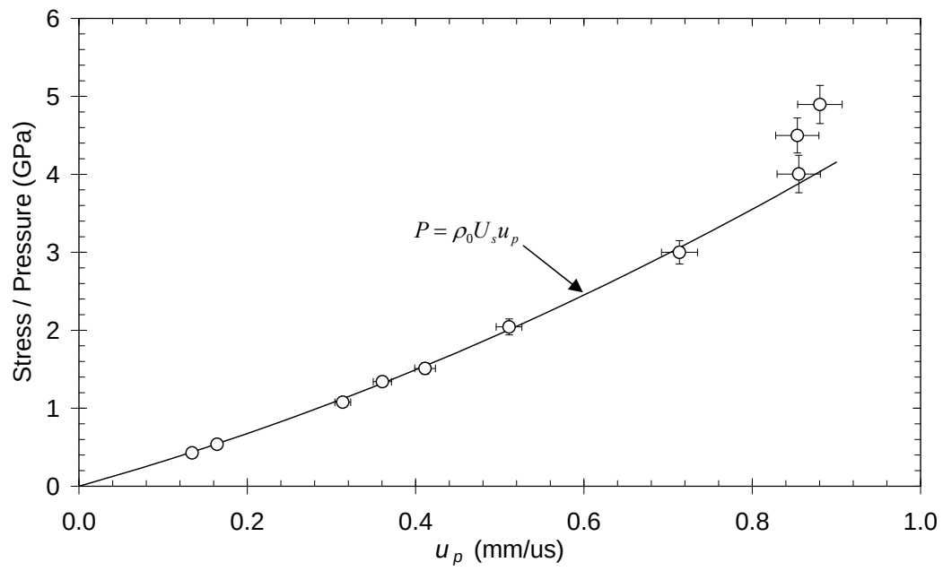
Figure 5: Stress – particle velocity Hugoniot plots for the resin.
