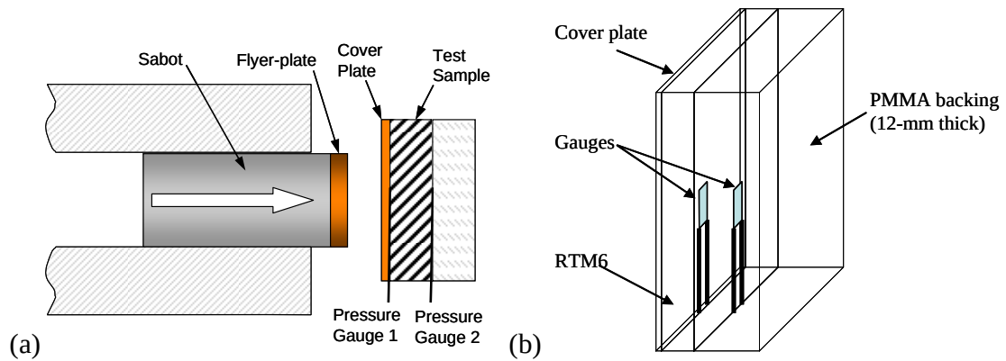
Figure 1: (a) the Flyer plate technique, (b) schematic target assembly
