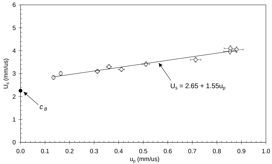
Figure 3: The measured Hugoniot of the resin in shock velocity particle velocity space.
