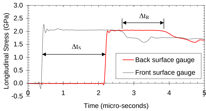
Figure 2: Typical gauge trace showing the formation of the shock and release.
