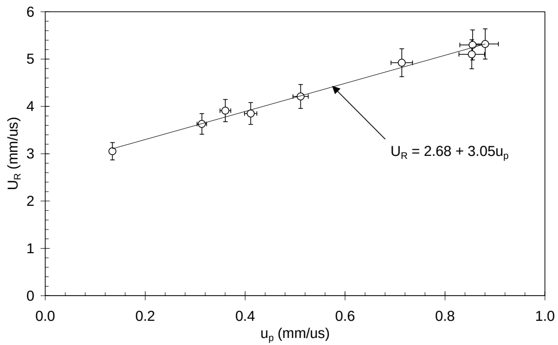
Figure 4: A plot of the calculated release wave velocities. One data point is omitted due to premature failure of one of the gauges in that experiment.
