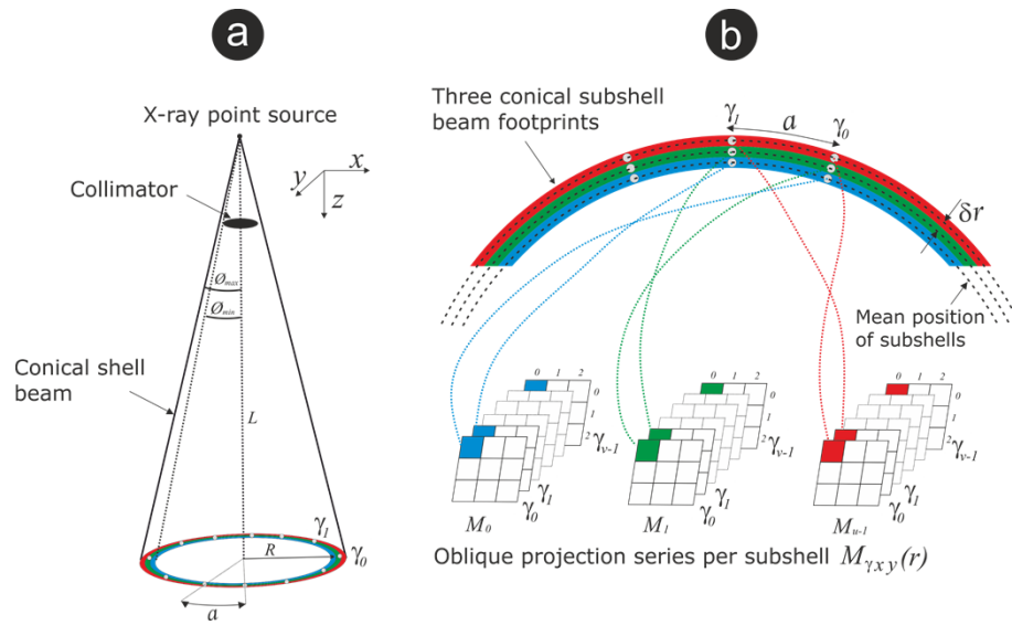
Fig. 1. (a) A schematic of a conical shell X-ray beam and incident annular footprint on a detection surface; where \phi_{\max/\min} are the outer/inner half-opening angles of the beam envelope, \gamma is the azimuth and ‘ a ’ is the incremental change in azimuth, L is the separation between the point source and the detection plane, and R is the mean radius of the innermost (blue) subshell on the detection plane. A phantom is raster scanned ( x, y ) through the beam (or equivalently vice versa) to enable a series of annular projections to be recorded. By registering the pixels sampled at their respective ( x, y ) positions in the scan, for a given azimuth and radial magnitude, an oblique (or inclined parallel) projection can be composited. Fig. (b) A schematic of an annular sector of the beam footprint (bounded by the inner and outer shell beam envelope) on the detection surface. In this example, the system is modelled as a series of three ‘color coded’ discrete concentric subshells centered on their mean radii (up to eight subshells are multiplexed during tomosynthesis in the experiments in this paper). The separation between a successive pair of radii is the minimum detectable radial increment \delta r . Thus, three different projection series M_{\gamma xy}(r) are collected from around their respective subshells. A specific series requires a constant magnitude of radial shift to effect a given axial focal plane position and requires appropriate multiplexing in the tomosynthesis.
