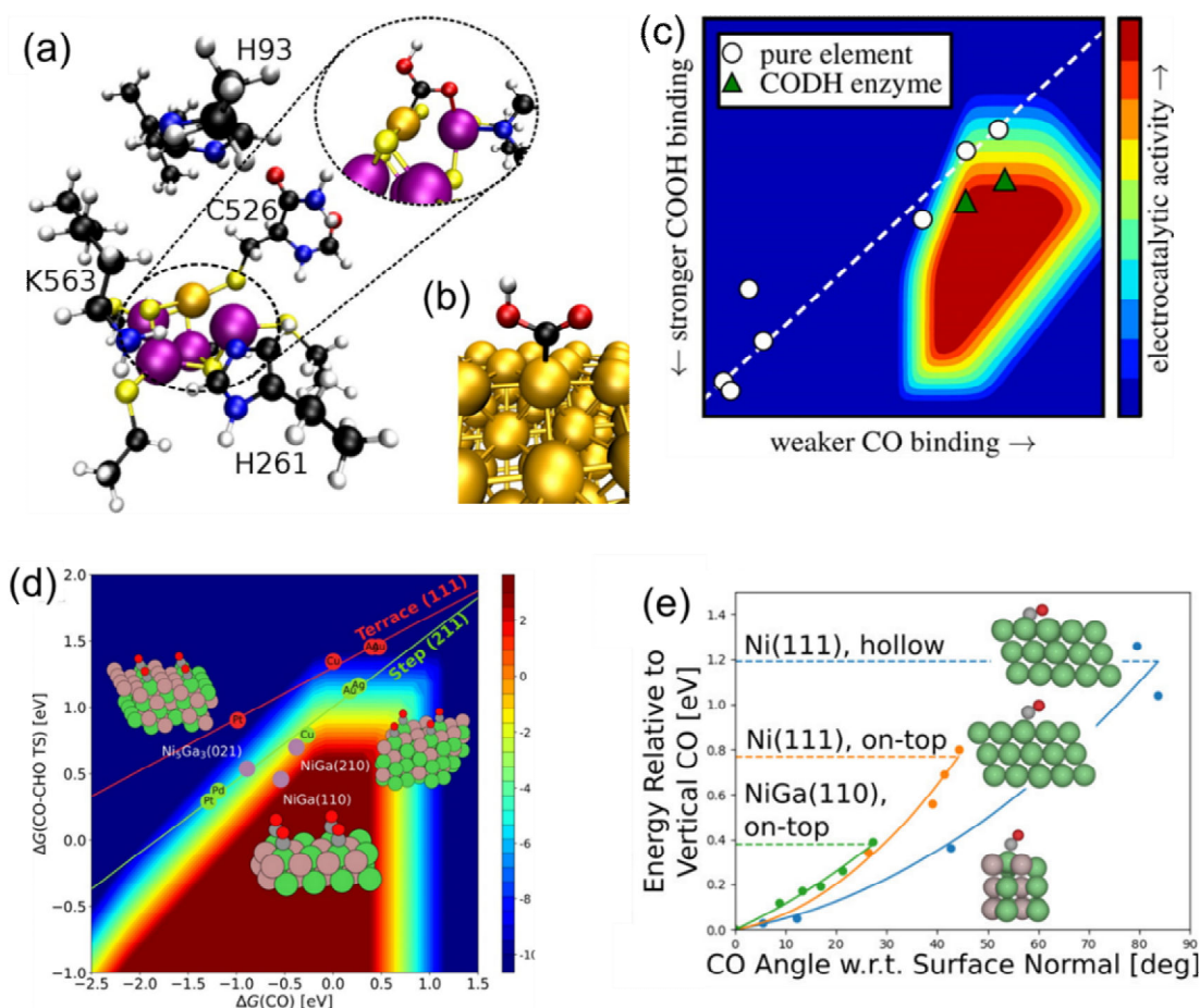
Fig. 1 Models of the active site for CO 2 electro-catalytic reduction on (a) enzyme and (b) Au surface. (c) Volcano activity plot for CO 2 electro-catalytic reduction at a 0.35 V overpotential. The data were obtained from the (211) stepped sites of transition metals. (d) Predicted activity of transition metal and the NiGa sites. (e) Rotation energy of CO on Ni and NiGa (110). Reprinted with permission from Refs. [24, 26].
