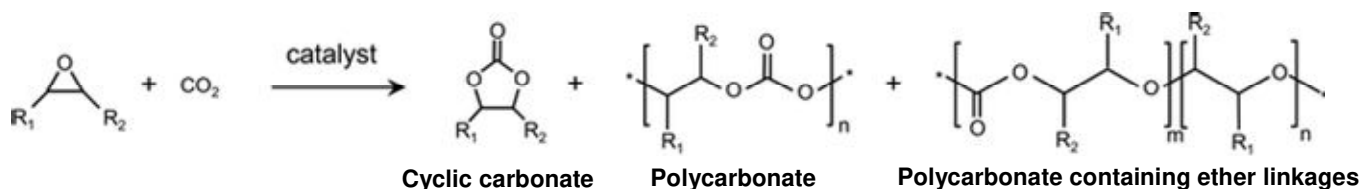
Fig. 2 Possible products from \text{CO}_2 reacting with epoxides. Reprinted with permission from Ref. [53].
