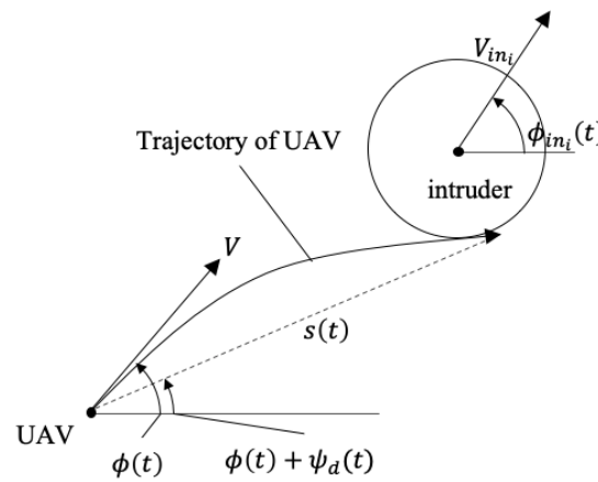
Figure 3. Collision avoidance geometry of a UAV to an intruder.
