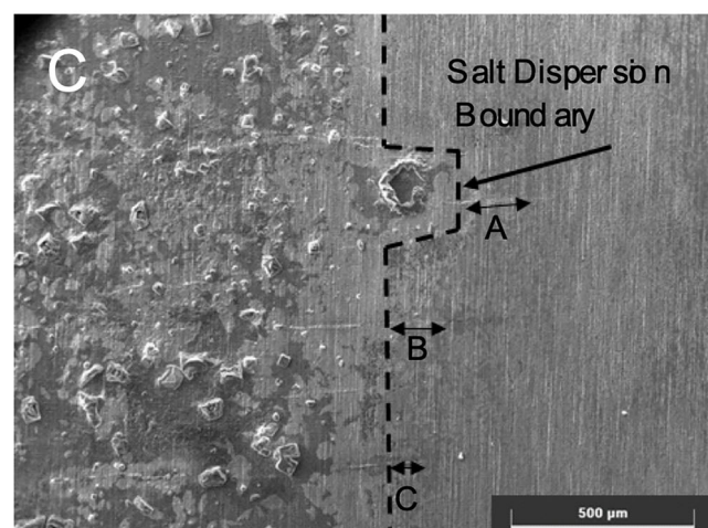
Fig. 8 | SEM images demonstrating. A standardized spacing between long cracks, which agrees with simulation results B, example of long cracks, and C positioning of the salt dispersion boundary and its role on total crack lengths. Some cracks are highlighted in red for better understanding.
