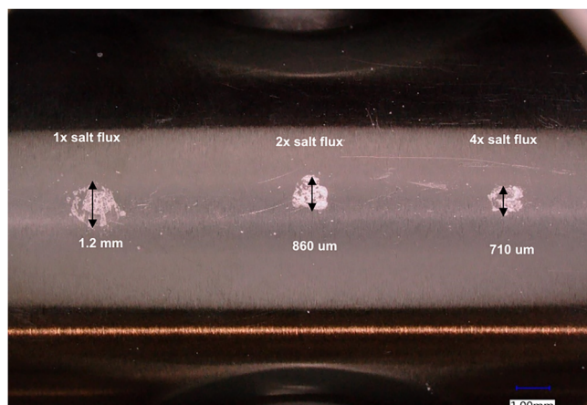
Fig. 12 | a Optical image showing the distribution of salt droplets for the pre-tested “One-Dot” C-ring.
