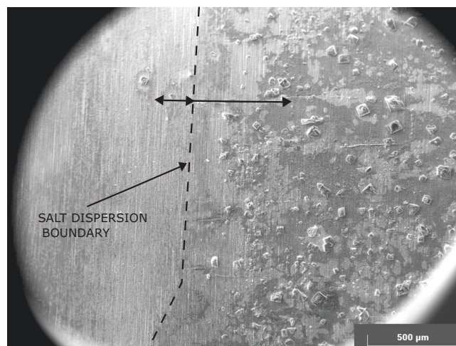
Fig. 9 | An example of an SEM image, which shows crack propagation quickly stagnating after passing the salt dispersion boundary.
