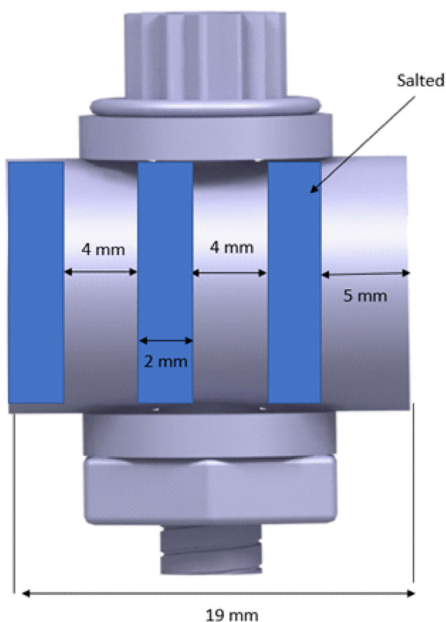
Fig. 6 | Zebra C-ring testing—schematic representation of the novel experimental configuration, designed to modify crack shielding. Shielding still occurs on the stripes, but not in between. Note the spacing between salted and unsalted regions.
