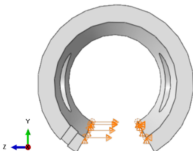
Fig. 4 | Schematic to represent how the boundary conditions are applied to the C-ring geometries. Triangles represent a pinned boundary condition, while arrows correspond to the applied displacement.
