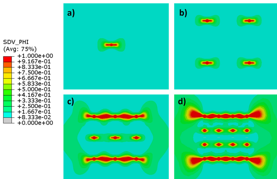
Fig. 2 | Schematic for the 2D simulations used to understand how the spacing between salt deposition sites may result in shorter or longer cracks. a–d Correspond to 1, 4, 9, and 16 salt deposition sites, respectively, in an array configuration.
