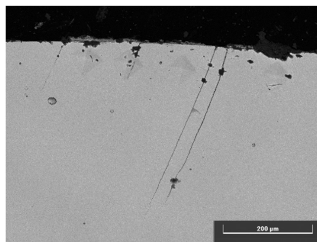
Fig. 10 | A through thickness microscopy image to show crack depths for a salted section of the c-ring.
