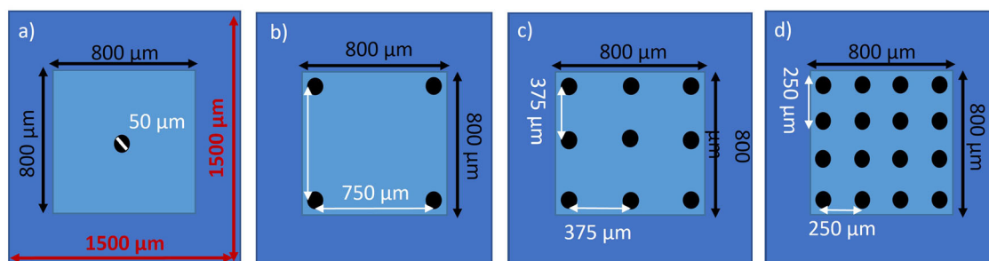
Fig. 2 | Schematic for the 2D simulations used to understand how the spacing between salt deposition sites may result in shorter or longer cracks. a–d Correspond to 1, 4, 9, and 16 salt deposition sites, respectively, in an array configuration.
