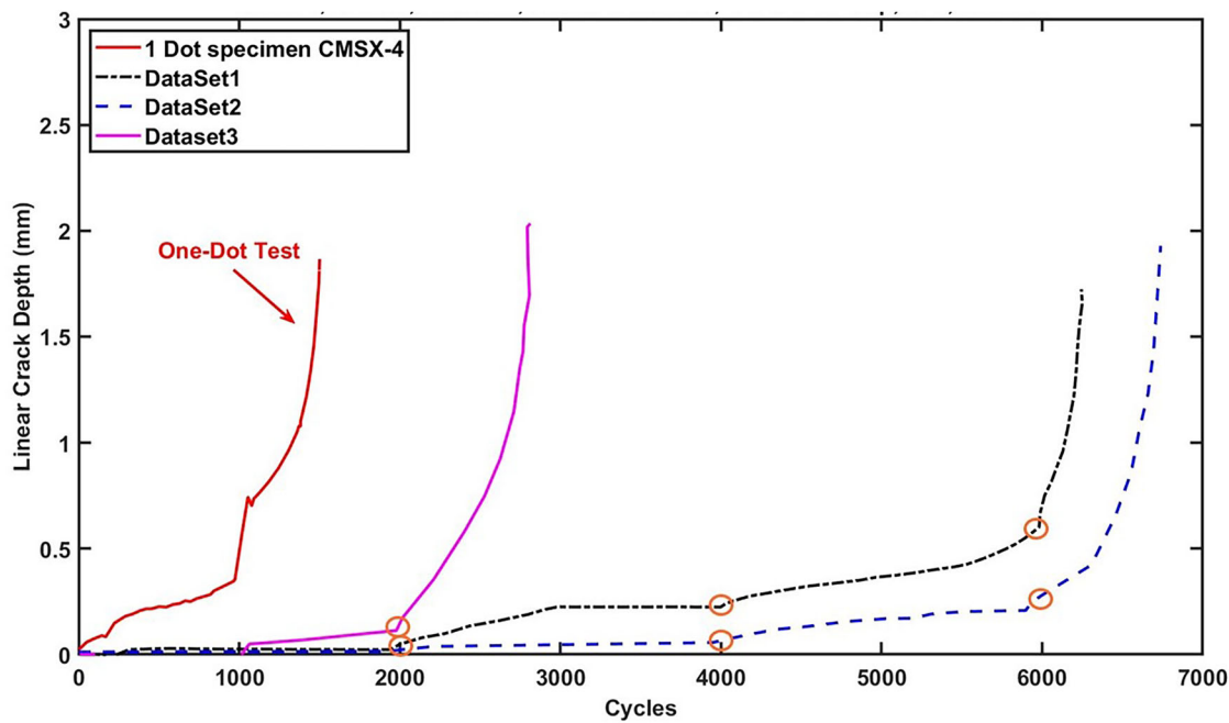
Fig. 17 | Plot highlighting the number of cycles needed to reach failure for a CMSX-4 corrosion-fatigue test, with the “One-Dot” test indicated by the red line. Please note that the 1-Dot test was NOT re-salted every 2000 cycles, unlike the other tests, which are highlighted using the orange circles.
