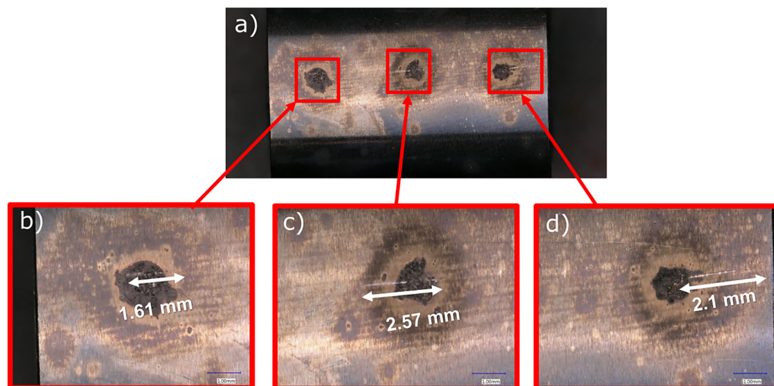
Fig. 13 | Optical images post testing of a C-ring with localized salt deposits. a Presents an overview to show the extent of cracking for each site of varying salt concentration while b , c and d representing 1x, 2x, and 4x salt flux respectively.
