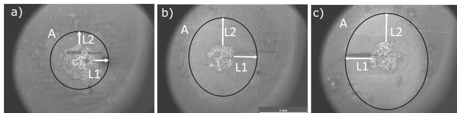
Fig. 14 | SEM images of the ‘Dot’ sample after testing. a–c Corresponds to varying salt flux (1.2 \mu\text{g}/\text{cm}^2/\text{h} , twice, and four times as much respectively). The analysis demonstrates that as salt flux increases the area of salt dispersion also increases.
