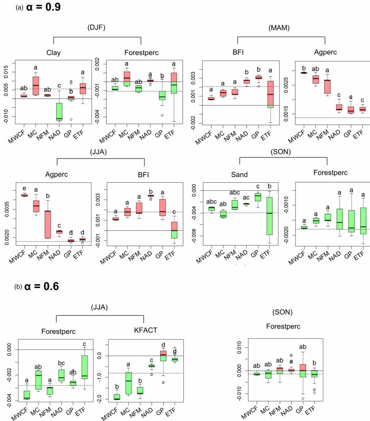
Figure 6 | GWR coefficients of duration of events (a, \alpha = 0.9 and b, \alpha = 0.6 ) (Log10 transformed): \alpha from Lyne and Hollick filter that larger value yielded longer duration of event. Forestperc is average percentage of forest cover. Sand is average percentage of sand. K-factor is average K-factor for upper most soil horizon. Please refer to the online version of this paper to see this figure in colour: http://dx.doi.org/10.2166/nh.2023.127 .
