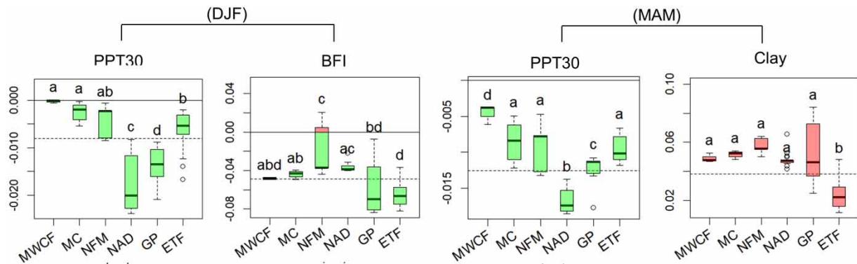
Figure 4 | GWR coefficients of M50 in different ecoregion (Log10 transformed): PPT30 is mean annual precipitation (1971–2000, cm). BFI is the average baseflow index (%). Clay is average percentage of soil clay content. Please refer to the online version of this paper to see this figure in colour: http://dx.doi.org/10.2166/nh.2023.127 .
