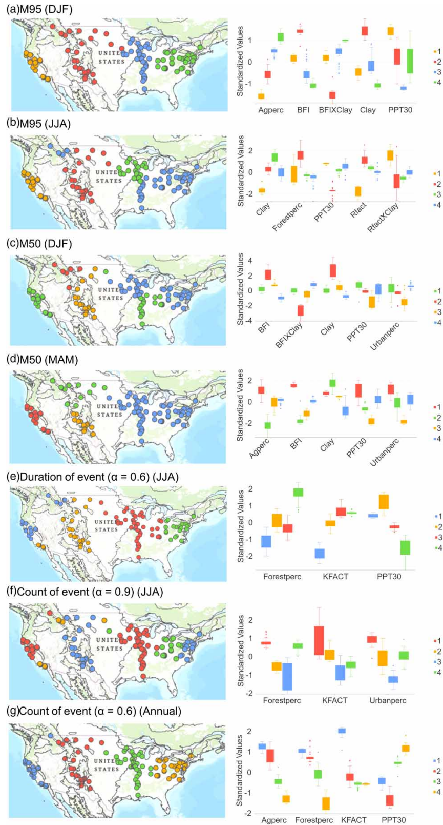
Figure 8 | A part of K-means clustering results (magnitude and frequency) on GWR coefficients from predictor variables in available distinctive seasons: four distinctive patterns were identified with the variables including BFI \times Clay . Please refer to the online version of this paper to see this figure in colour: http://dx.doi.org/10.2166/nh.2023.127 .
