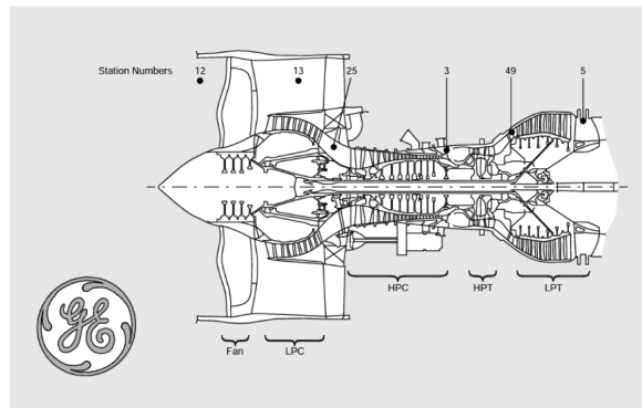
Figure 7: GE90-115B [18]
