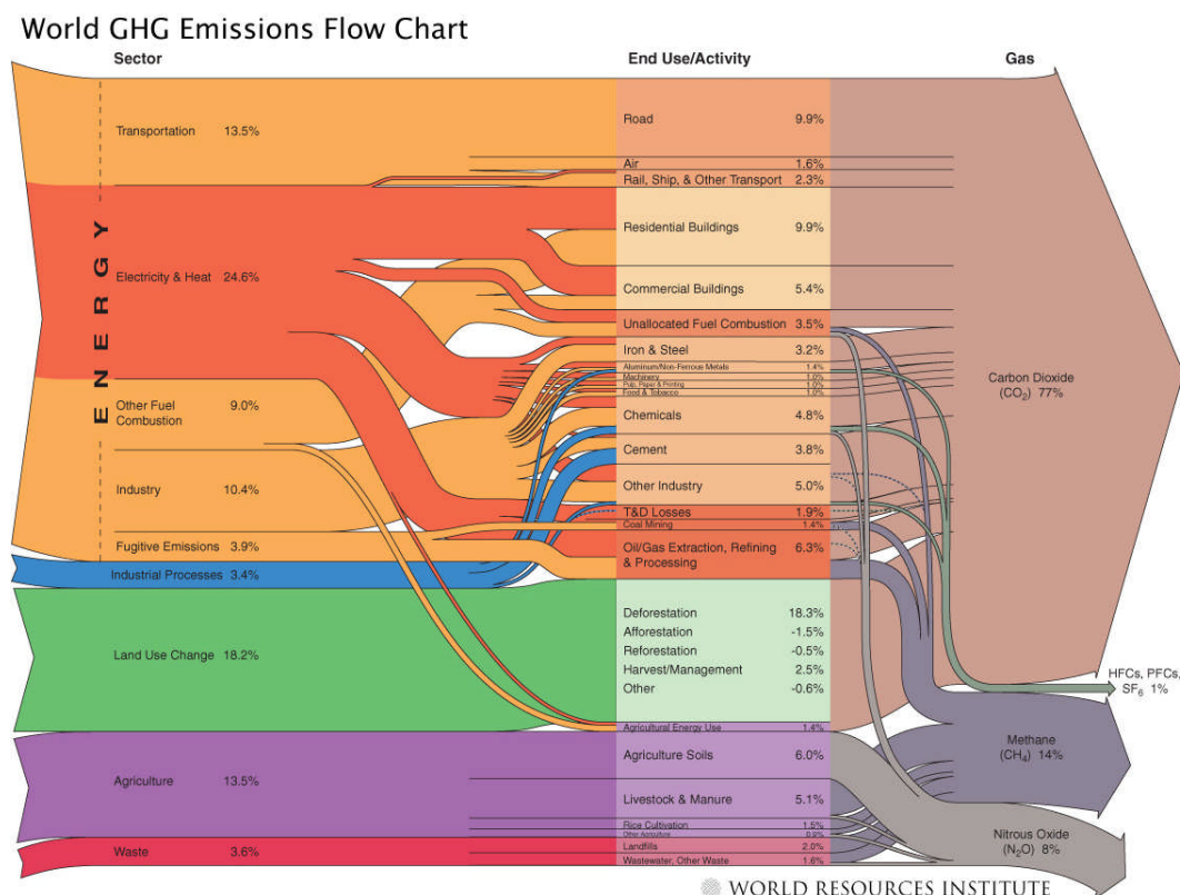
Figure 1. Flow of global greenhouse gas emissions
