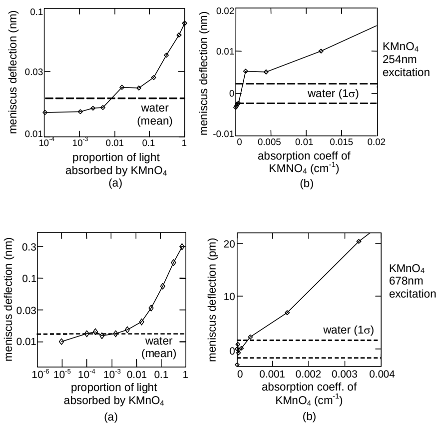
Figure 5. Photothermal signals resulting from absorption of light by KMnO 4 solutions from the UV lamp and the red laser diode. (a) Raw data. The dashed line shows the mean signal for a deionised water blank. (b) Following subtraction of the mean signal for deionised water (expanded scale). The dashed line shows one standard deviation in the signals for a deionised water blank.
