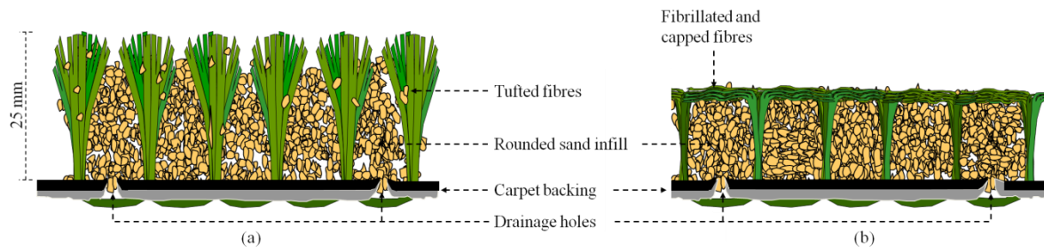
Figure 2 Fibrillation and capping of fibres in a worn synthetic turf surface – typically caused by insufficient depth of infill.
