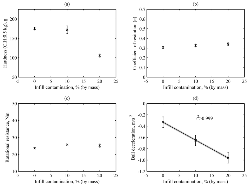
Figure 6. The effect of infill contamination on surface performance at 25 kg/m 2 of sand infill: (a) hardness as determined by the 0.5 kg Clegg impact hammer (CIH); (b) coefficient of restitution for a standard hockey ball dropped from 1.5 m; rotational resistance of a dimpled rubber sole; (d) deceleration of a hockey ball over 1 m released from 1 m height down a 45° ramp. Values are means, with whiskers representing the standard error of the mean. Solid lines represent the linear regression model for the mean data where p < 0.05 ; dashed lines are the 95% confidence intervals of the linear model, r^2 represents the coefficient of determination.
